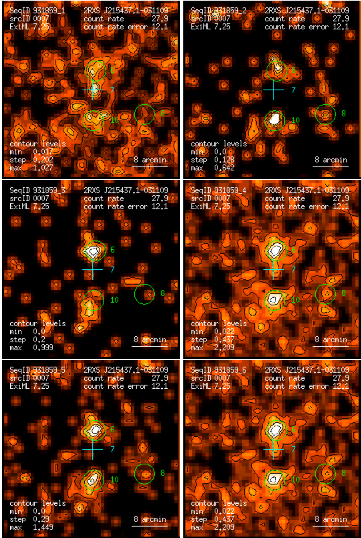
Figure 7: RASS 931859: detection 0007: band rate images, Gaussian filter: (1) PSPC channels 11 – 41, (2) 52 – 90, (3) 91 – 201, (4) 11 – 235, (5) 52 – 201, (6) 11 – 201. Broad band rates in counts/ks. Band rate contour levels in counts/ks/arcmin 2 .
