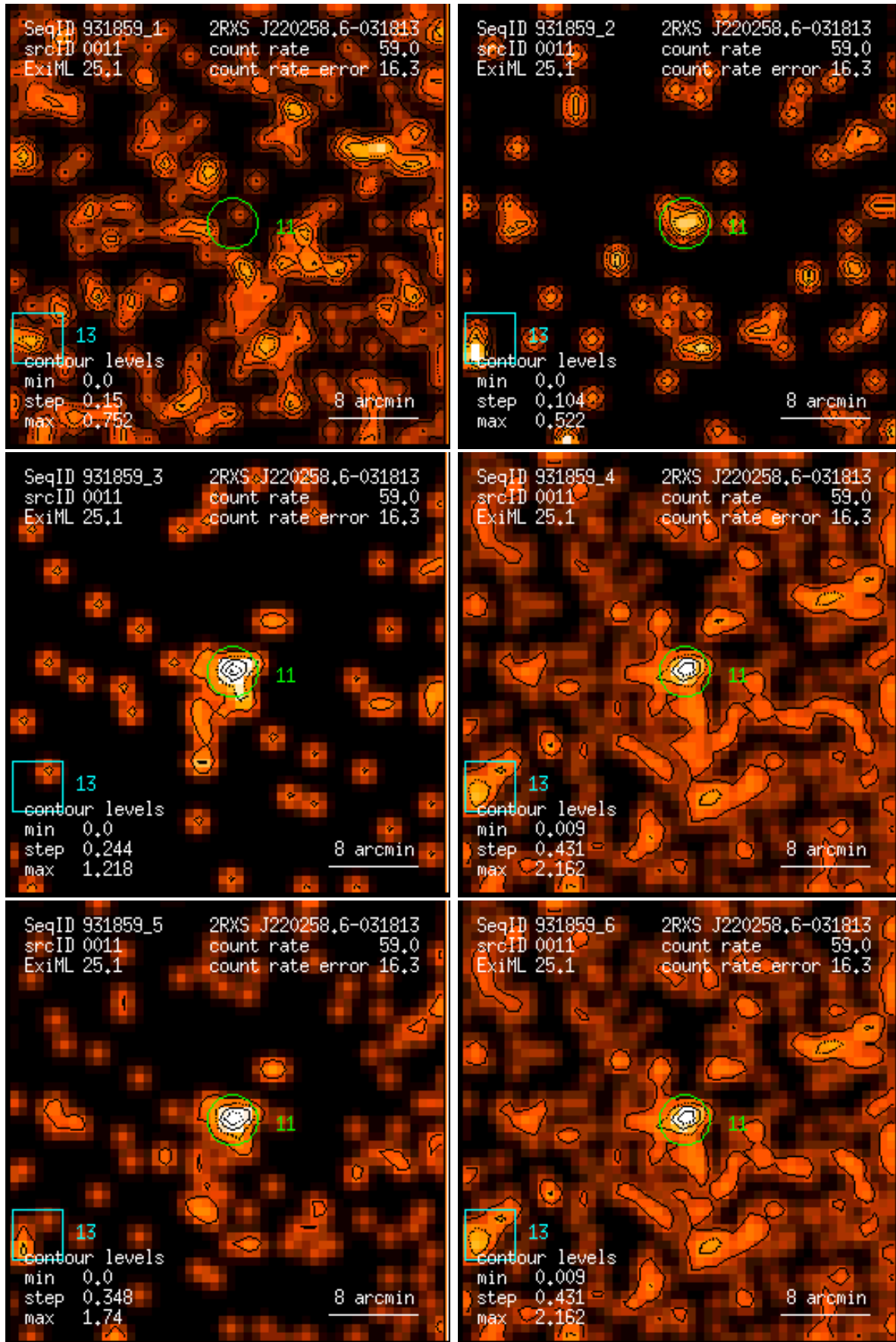
Figure 11: RASS 931859: detection 0011: band rate images, Gaussian filter: (1) PSPC channels 11 – 41, (2) 52 – 90, (3) 91 – 201, (4) 11 – 235, (5) 52 – 201, (6) 11 – 201. Broad band rates in counts/ks. Band rate contour levels in counts/ks/arcmin 2 .
