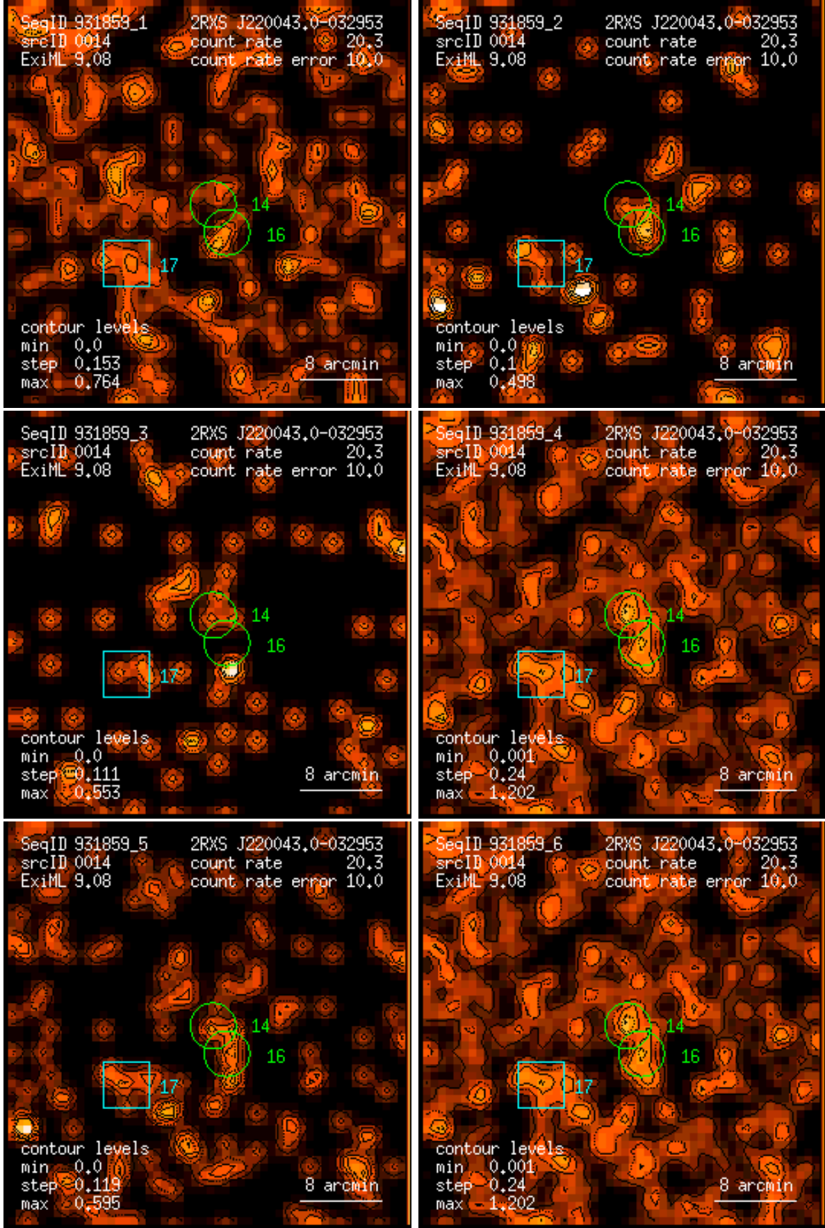
Figure 14: RASS 931859: detection 0014: band rate images, Gaussian filter: (1) PSPC channels 11 – 41, (2) 52 – 90, (3) 91 – 201, (4) 11 – 235, (5) 52 – 201, (6) 11 – 201. Broad band rates in counts/ks. Band rate contour levels in counts/ks/arcmin 2 .
