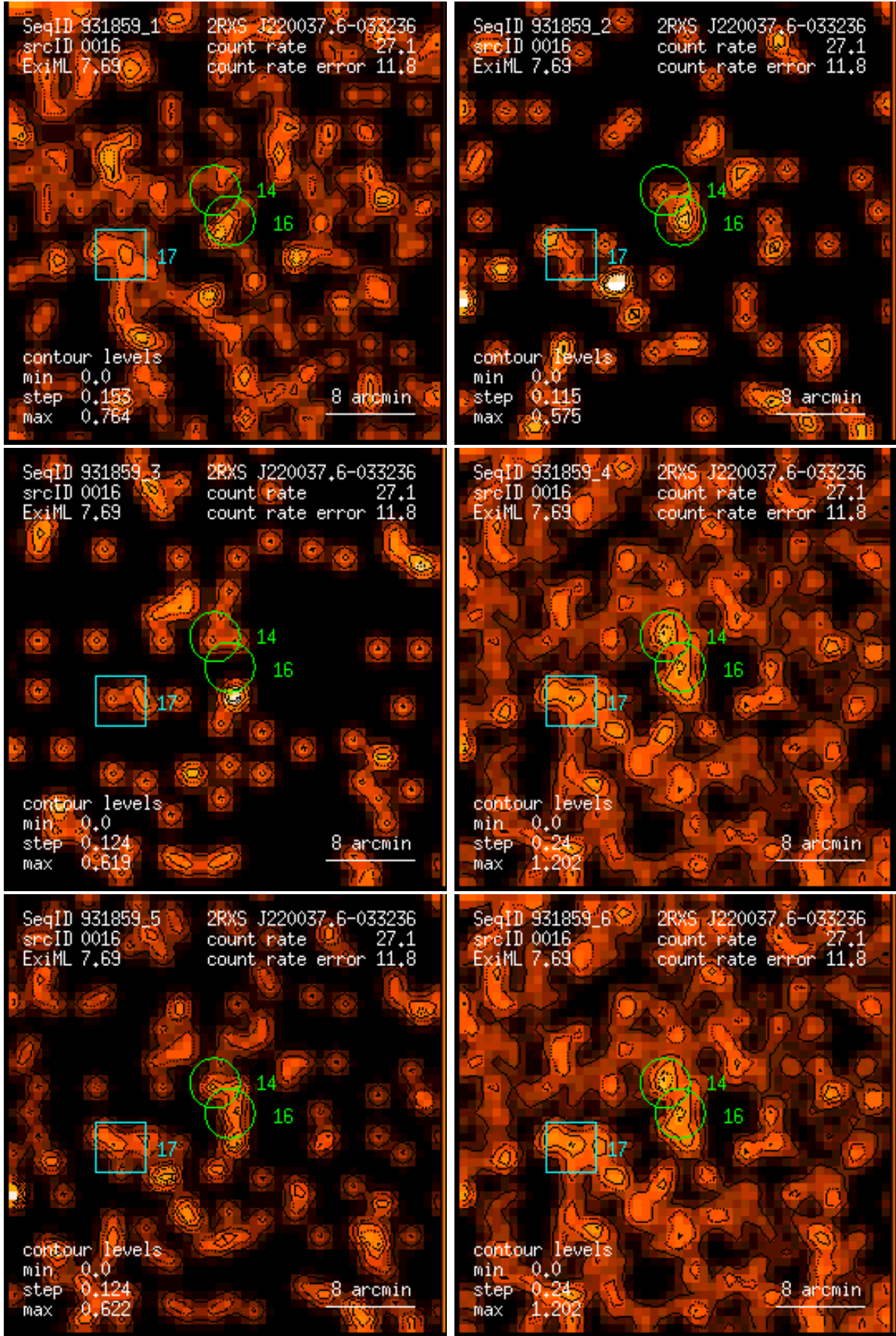
Figure 16: RASS 931859: detection 0016: band rate images, Gaussian filter: (1) PSPC channels 11 – 41, (2) 52 – 90, (3) 91 – 201, (4) 11 – 235, (5) 52 – 201, (6) 11 – 201. Broad band rates in counts/ks. Band rate contour levels in counts/ks/arcmin 2 .
