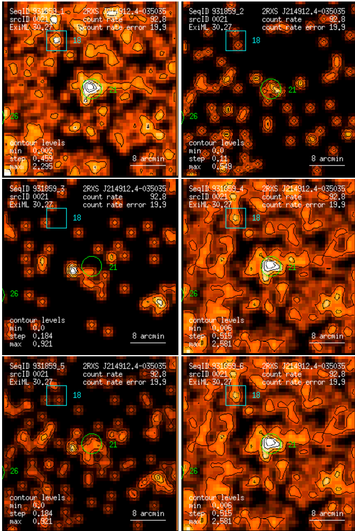
Figure 21: RASS 931859: detection 0021: band rate images, Gaussian filter: (1) PSPC channels 11 – 41, (2) 52 – 90, (3) 91 – 201, (4) 11 – 235, (5) 52 – 201, (6) 11 – 201. Broad band rates in counts/ks. Band rate contour levels in counts/ks/arcmin 2 .
