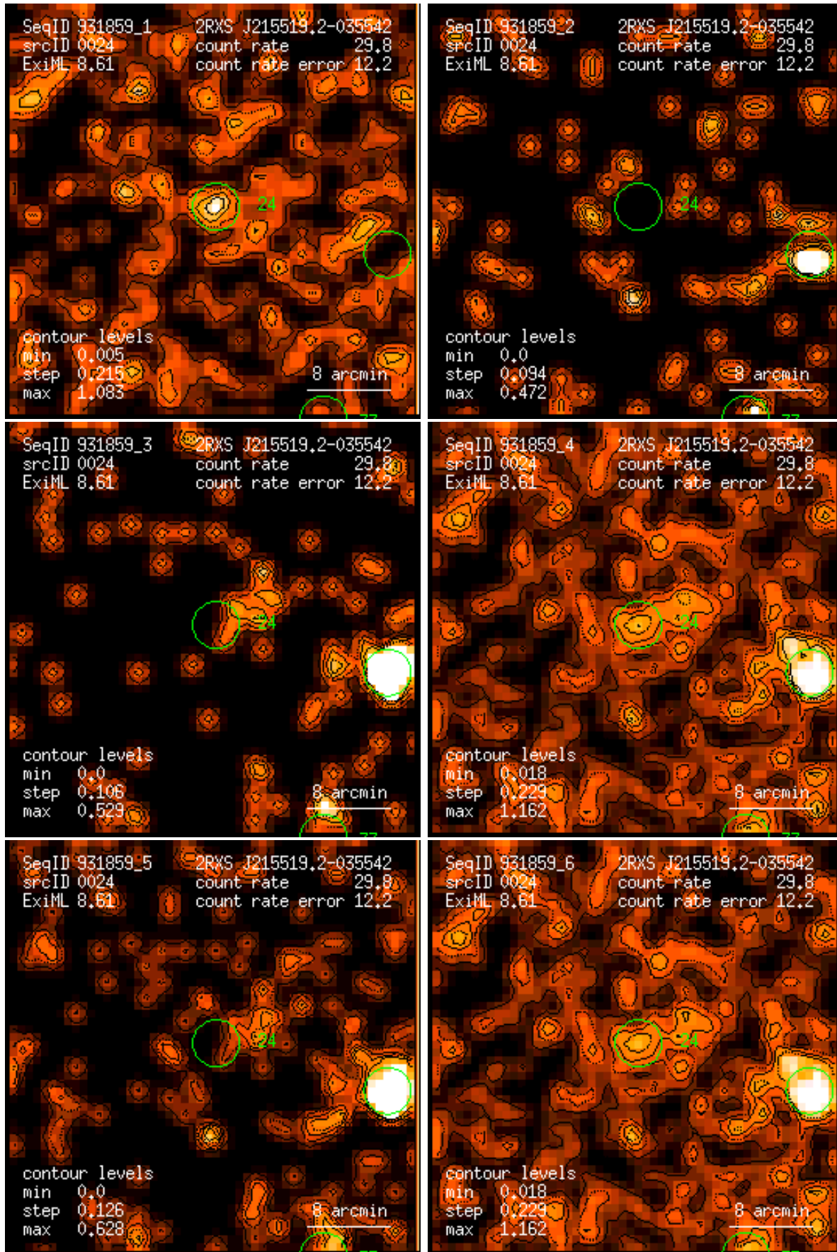
Figure 24: RASS 931859: detection 0024: band rate images, Gaussian filter: (1) PSPC channels 11 – 41, (2) 52 – 90, (3) 91 – 201, (4) 11 – 235, (5) 52 – 201, (6) 11 – 201. Broad band rates in counts/ks. Band rate contour levels in counts/ks/arcmin 2 .
