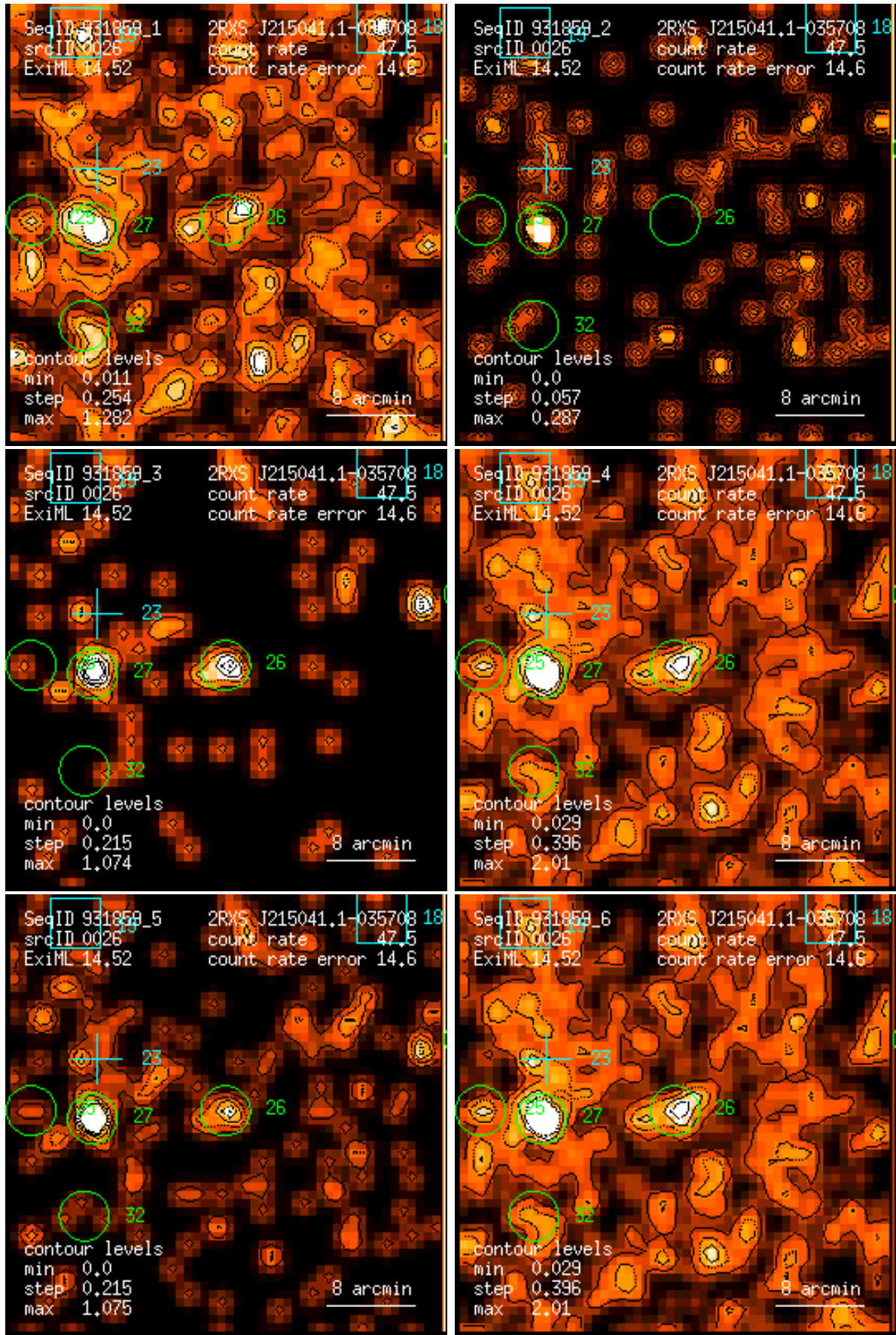
Figure 26: RASS 931859: detection 0026: band rate images, Gaussian filter: (1) PSPC channels 11 – 41, (2) 52 – 90, (3) 91 – 201, (4) 11 – 235, (5) 52 – 201, (6) 11 – 201. Broad band rates in counts/ks. Band rate contour levels in counts/ks/arcmin 2 .
