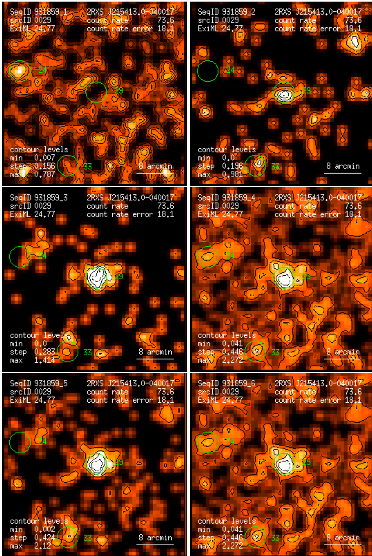
Figure 29: RASS 931859: detection 0029: band rate images, Gaussian filter: (1) PSPC channels 11 – 41, (2) 52 – 90, (3) 91 – 201, (4) 11 – 235, (5) 52 – 201, (6) 11 – 201. Broad band rates in counts/ks. Band rate contour levels in counts/ks/arcmin 2 .
