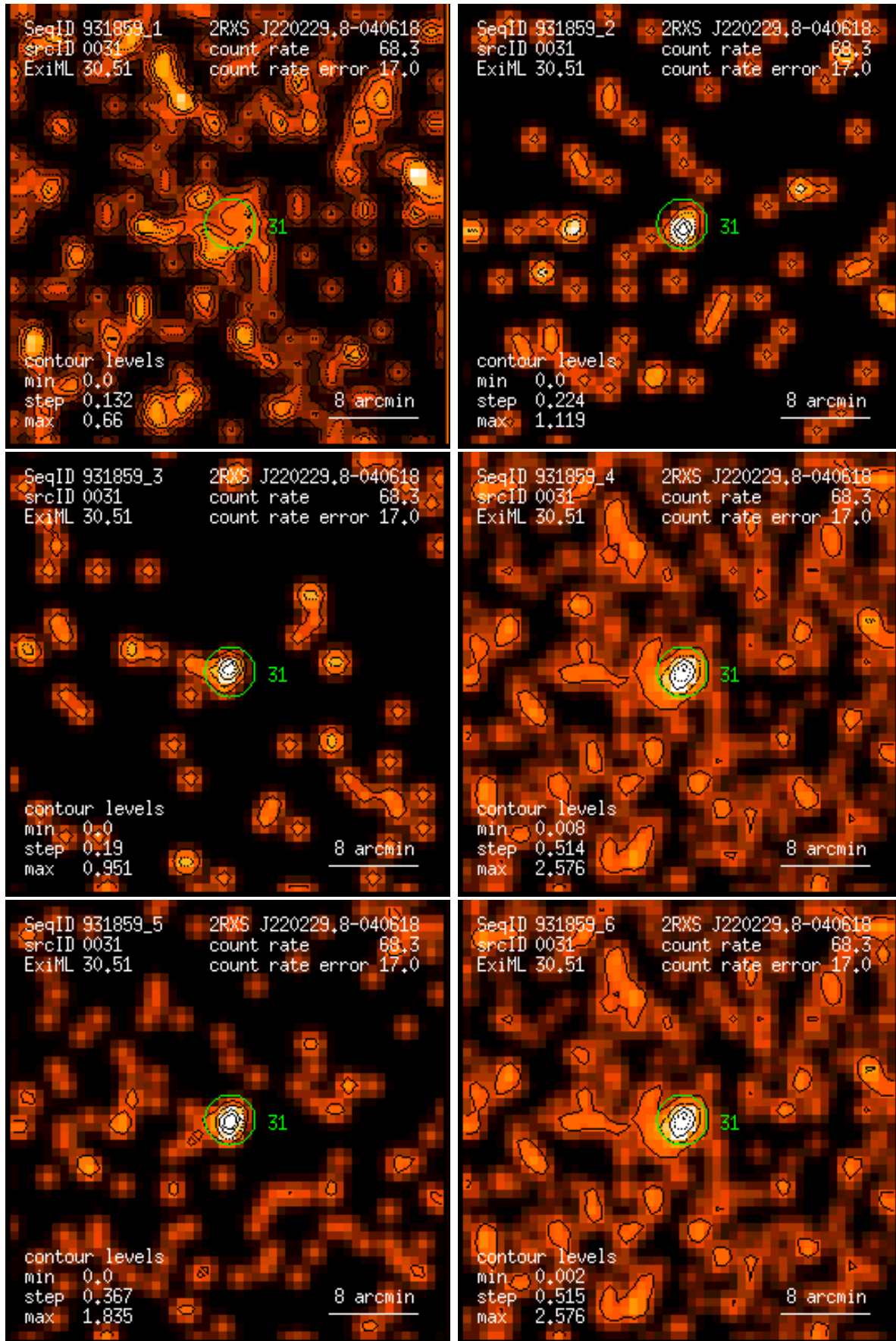
Figure 31: RASS 931859: detection 0031: band rate images, Gaussian filter: (1) PSPC channels 11 – 41, (2) 52 – 90, (3) 91 – 201, (4) 11 – 235, (5) 52 – 201, (6) 11 – 201. Broad band rates in counts/ks. Band rate contour levels in counts/ks/arcmin 2 .
