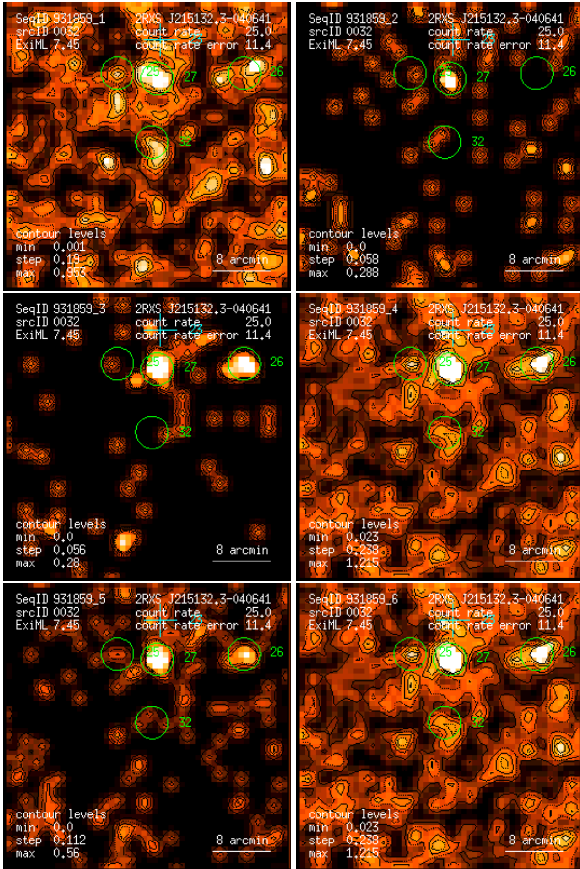
Figure 32: RASS 931859: detection 0032: band rate images, Gaussian filter: (1) PSPC channels 11 – 41, (2) 52 – 90, (3) 91 – 201, (4) 11 – 235, (5) 52 – 201, (6) 11 – 201. Broad band rates in counts/ks. Band rate contour levels in counts/ks/arcmin 2 .
