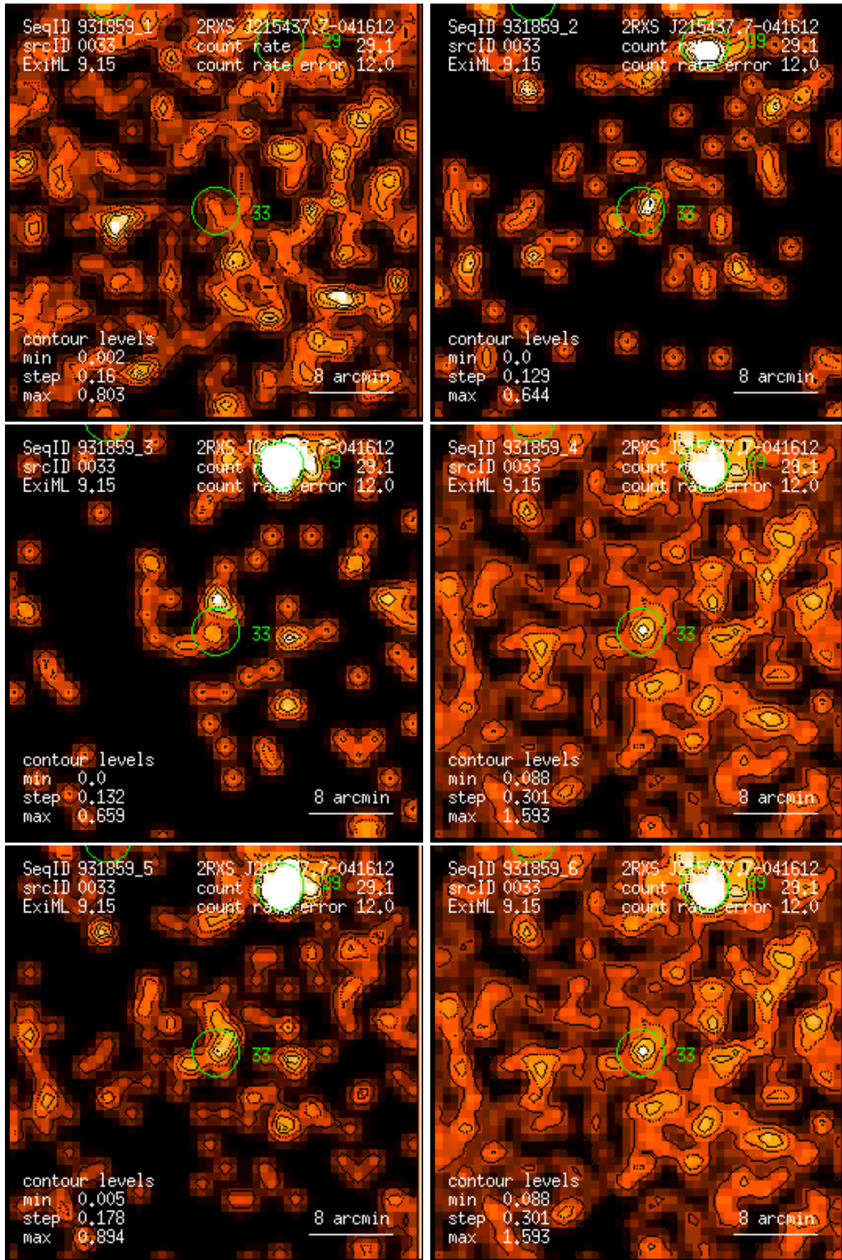
Figure 33: RASS 931859: detection 0033: band rate images, Gaussian filter: (1) PSPC channels 11 – 41, (2) 52 – 90, (3) 91 – 201, (4) 11 – 235, (5) 52 – 201, (6) 11 – 201. Broad band rates in counts/ks. Band rate contour levels in counts/ks/arcmin 2 .
