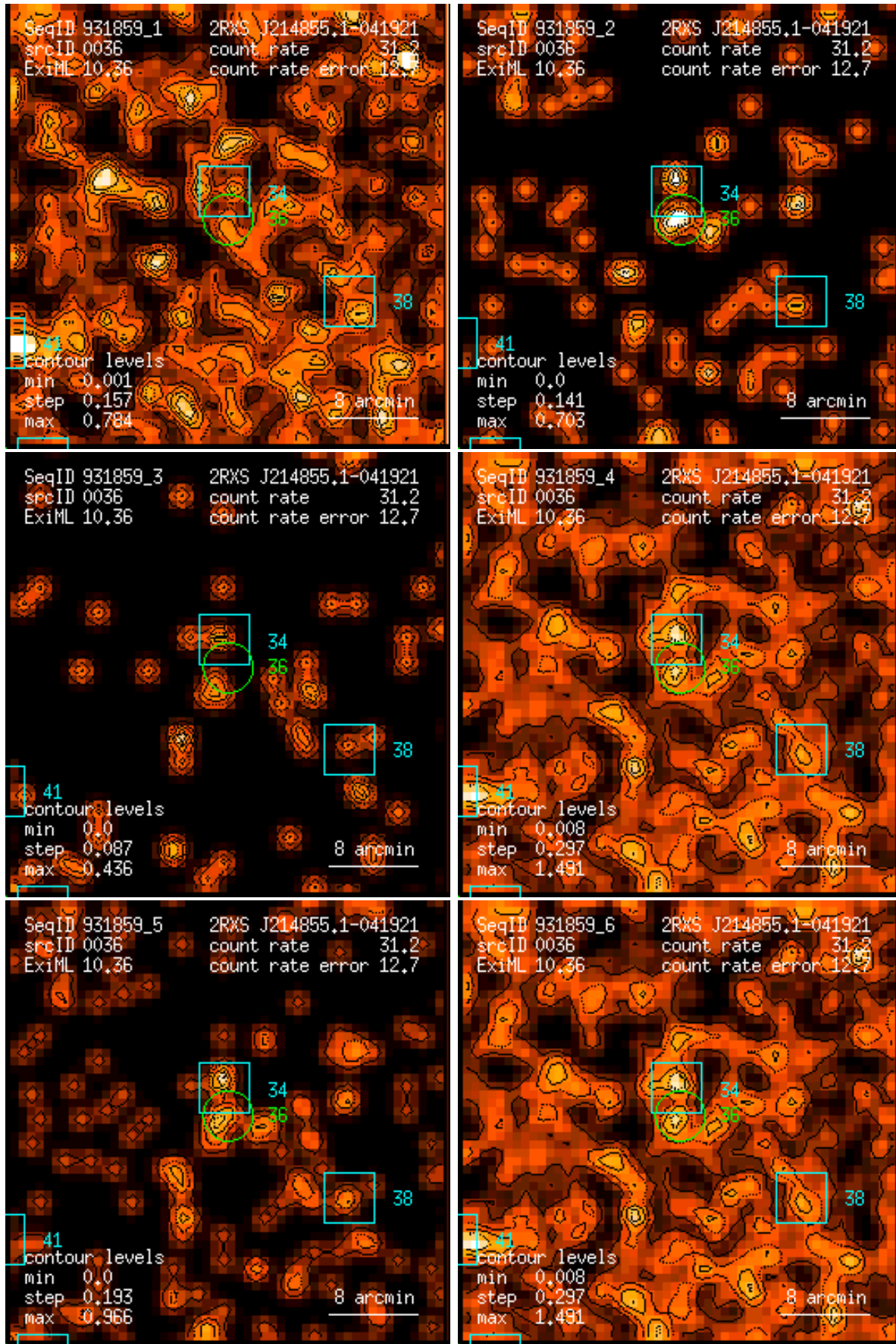
Figure 36: RASS 931859: detection 0036: band rate images, Gaussian filter: (1) PSPC channels 11 – 41, (2) 52 – 90, (3) 91 – 201, (4) 11 – 235, (5) 52 – 201, (6) 11 – 201. Broad band rates in counts/ks. Band rate contour levels in counts/ks/arcmin 2 .
