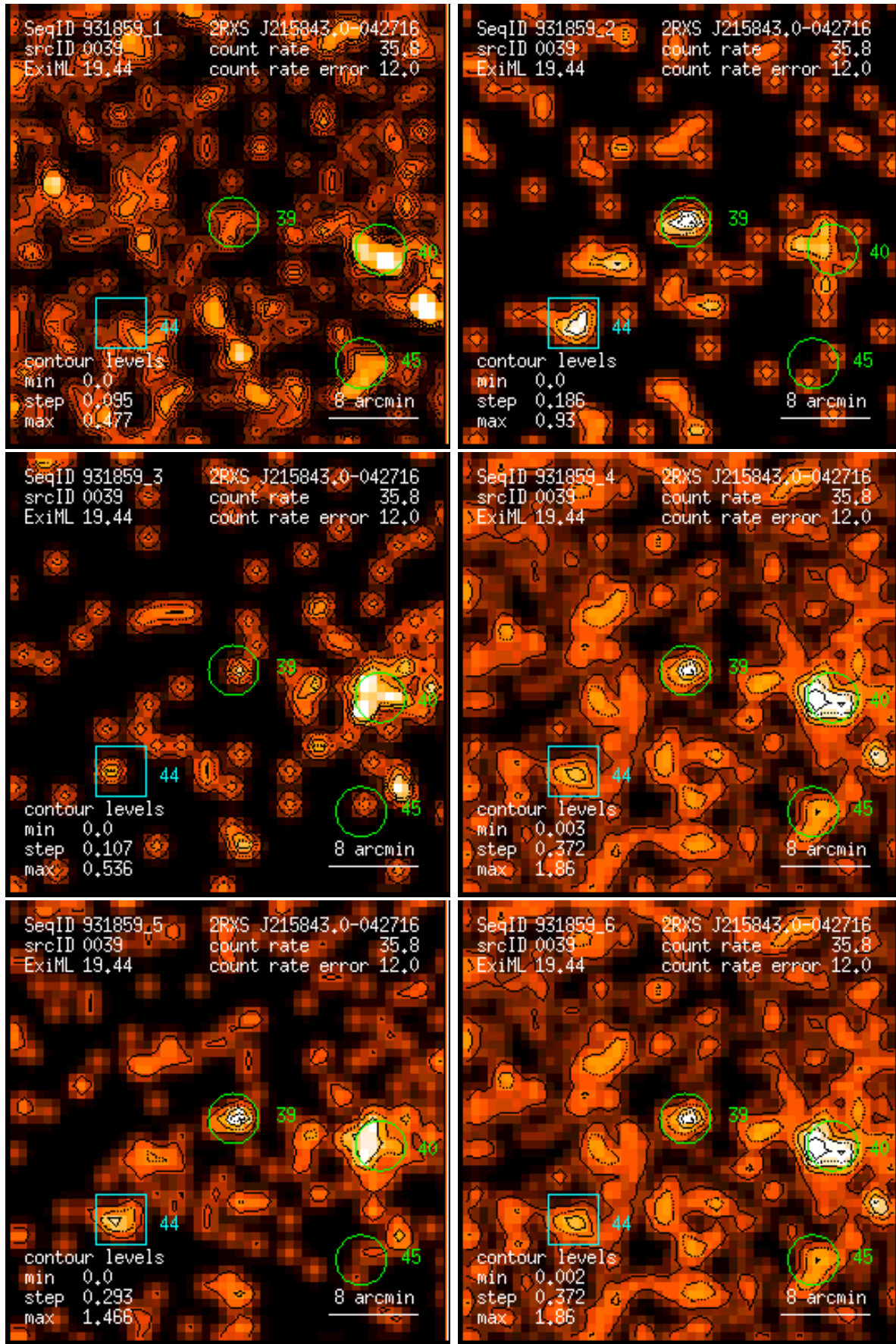
Figure 39: RASS 931859: detection 0039: band rate images, Gaussian filter: (1) PSPC channels 11 – 41, (2) 52 – 90, (3) 91 – 201, (4) 11 – 235, (5) 52 – 201, (6) 11 – 201. Broad band rates in counts/ks. Band rate contour levels in counts/ks/arcmin 2 .
