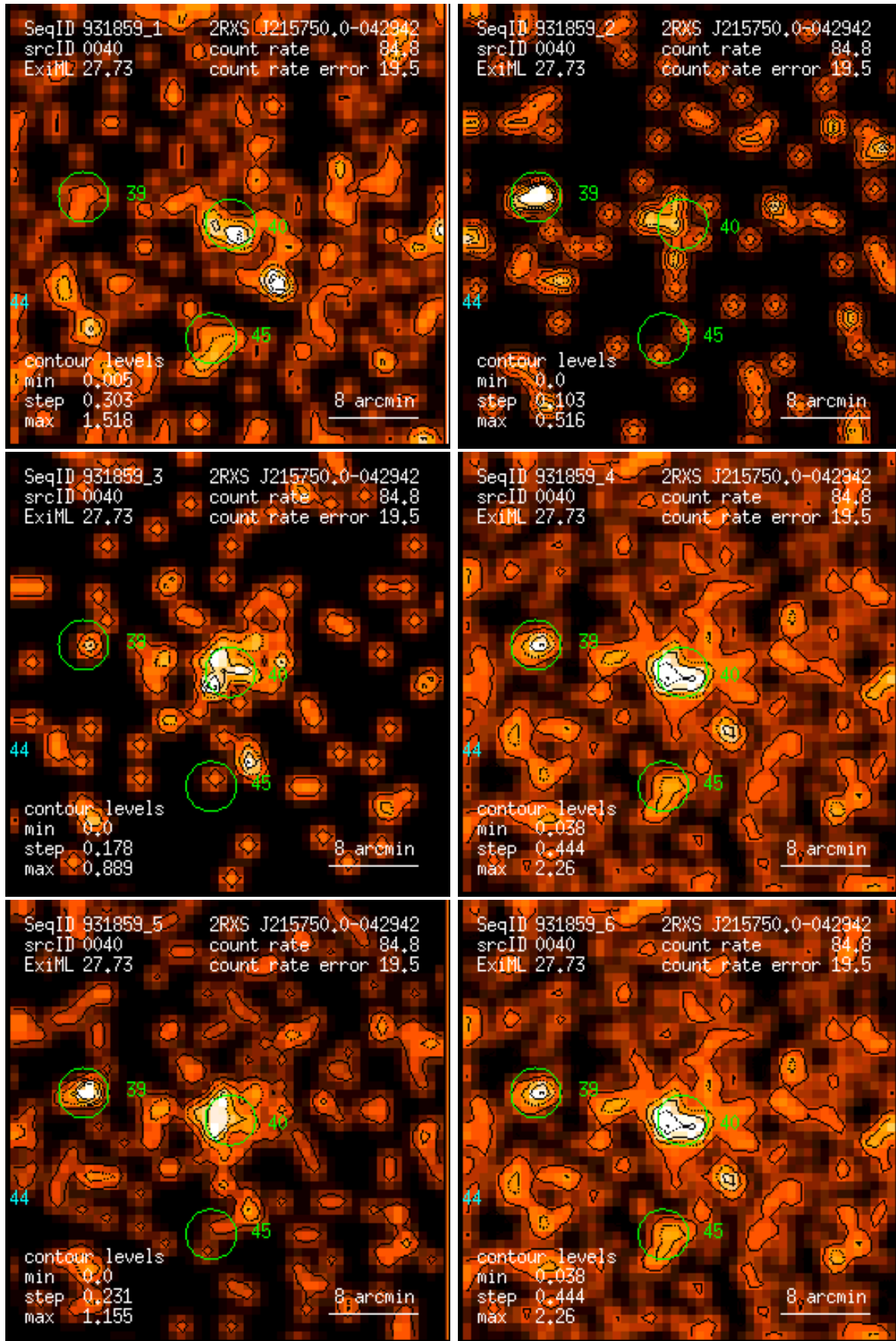
Figure 40: RASS 931859: detection 0040: band rate images, Gaussian filter: (1) PSPC channels 11 – 41, (2) 52 – 90, (3) 91 – 201, (4) 11 – 235, (5) 52 – 201, (6) 11 – 201. Broad band rates in counts/ks. Band rate contour levels in counts/ks/arcmin 2 .
