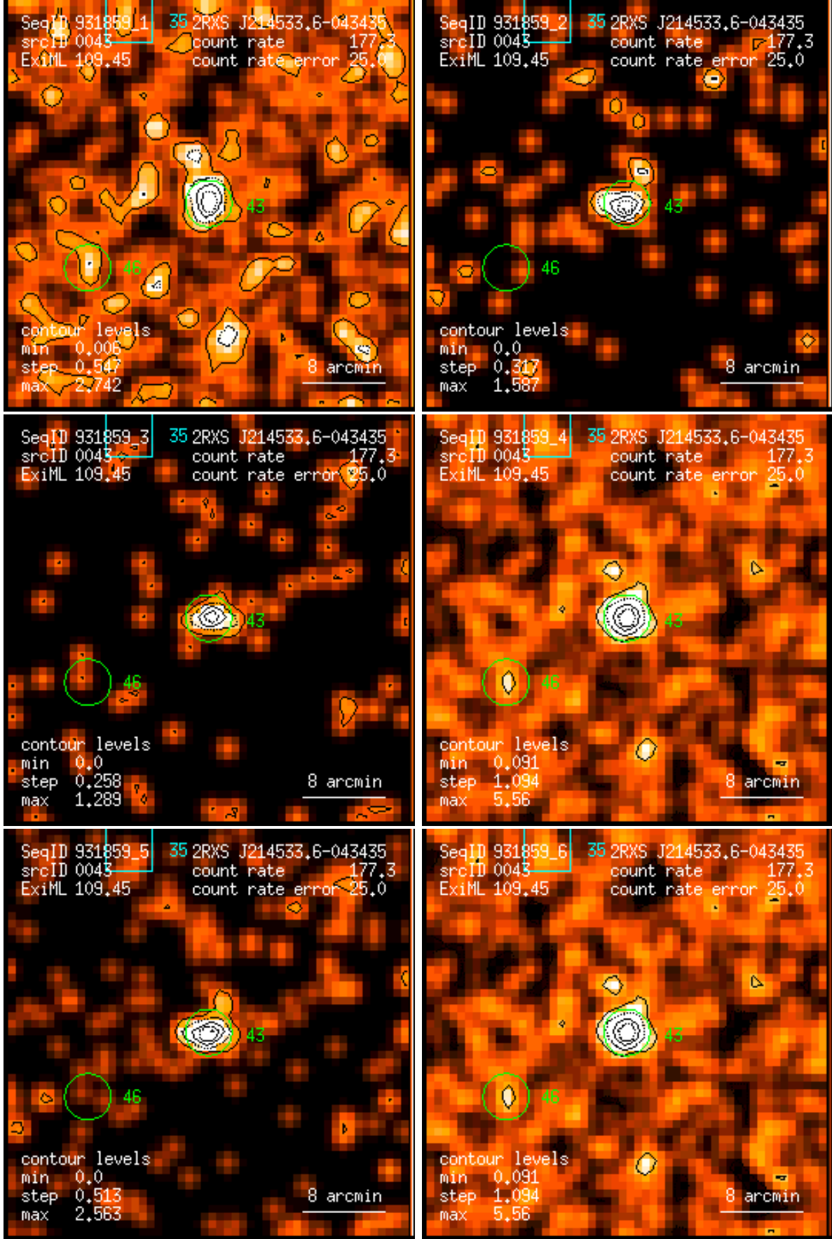
Figure 43: RASS 931859: detection 0043: band rate images, Gaussian filter: (1) PSPC channels 11 – 41, (2) 52 – 90, (3) 91 – 201, (4) 11 – 235, (5) 52 – 201, (6) 11 – 201. Broad band rates in counts/ks. Band rate contour levels in counts/ks/arcmin 2 .
