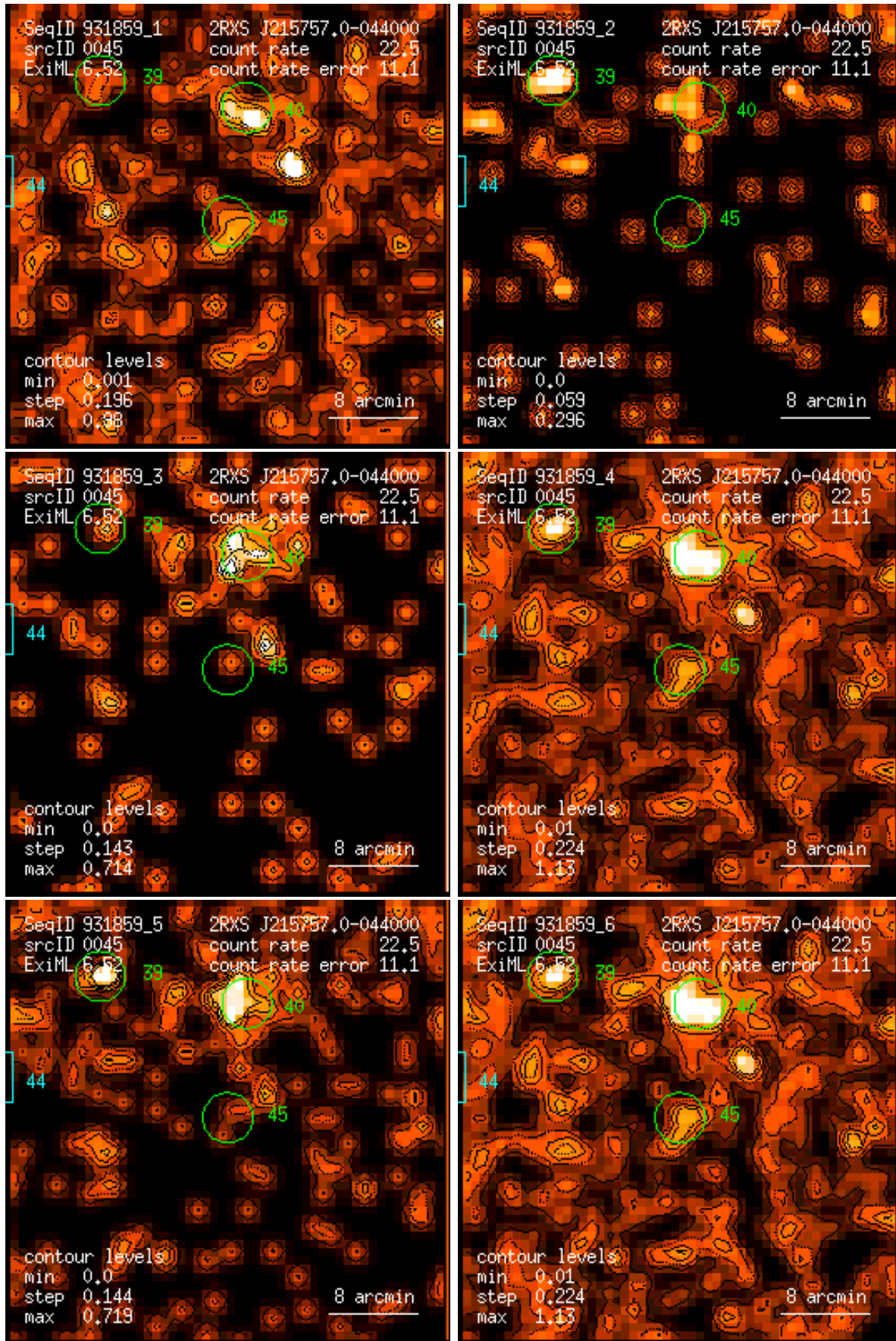
Figure 45: RASS 931859: detection 0045: band rate images, Gaussian filter: (1) PSPC channels 11 – 41, (2) 52 – 90, (3) 91 – 201, (4) 11 – 235, (5) 52 – 201, (6) 11 – 201. Broad band rates in counts/ks. Band rate contour levels in counts/ks/arcmin 2 .
