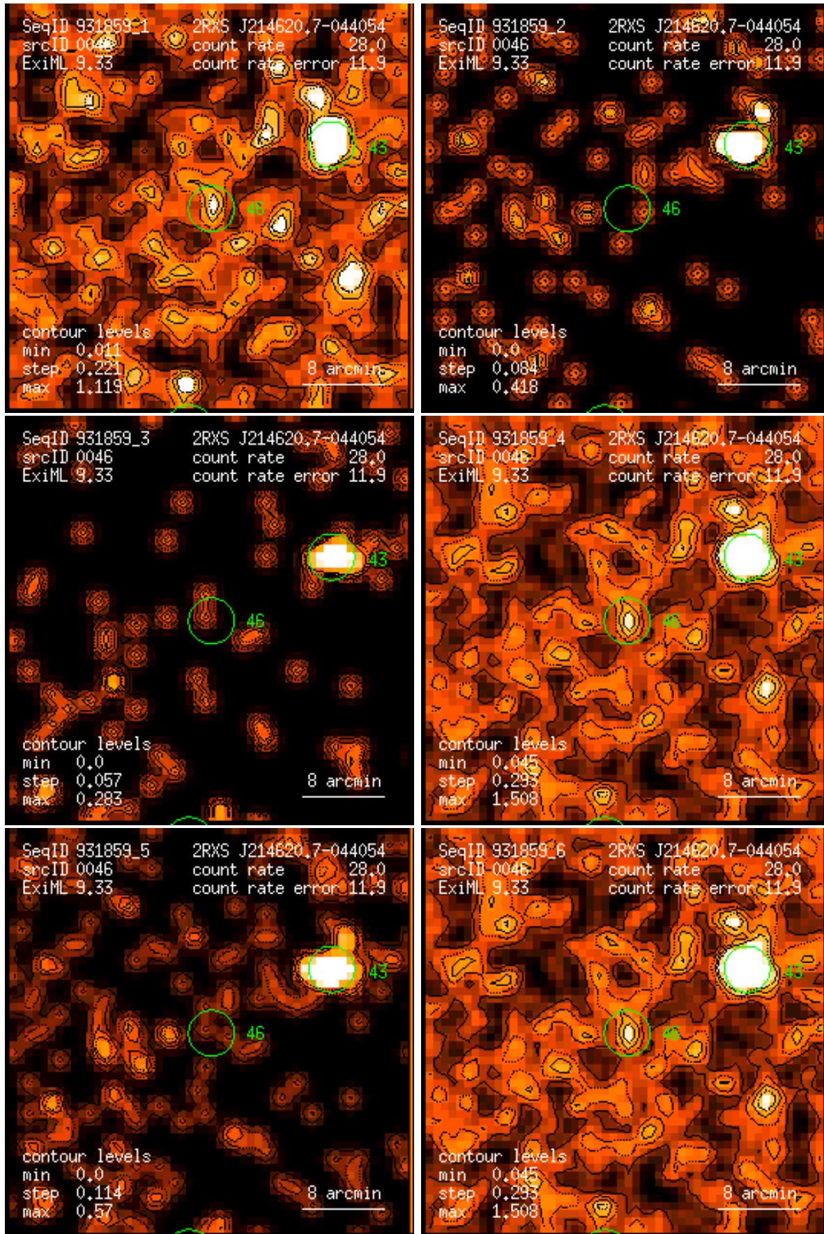
Figure 46: RASS 931859: detection 0046: band rate images, Gaussian filter: (1) PSPC channels 11 – 41, (2) 52 – 90, (3) 91 – 201, (4) 11 – 235, (5) 52 – 201, (6) 11 – 201. Broad band rates in counts/ks. Band rate contour levels in counts/ks/arcmin 2 .
