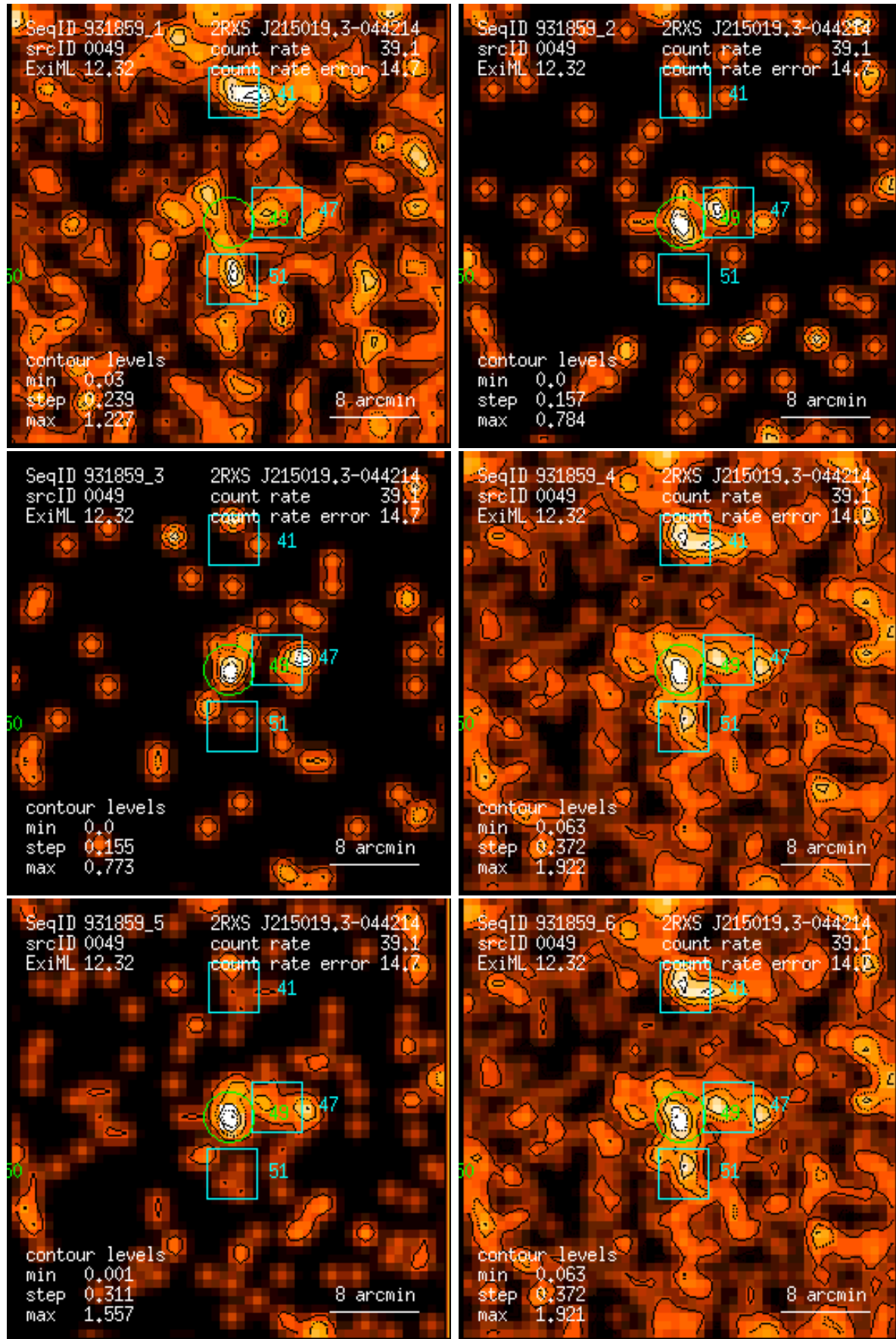
Figure 49: RASS 931859: detection 0049: band rate images, Gaussian filter: (1) PSPC channels 11 – 41, (2) 52 – 90, (3) 91 – 201, (4) 11 – 235, (5) 52 – 201, (6) 11 – 201. Broad band rates in counts/ks. Band rate contour levels in counts/ks/arcmin 2 .
