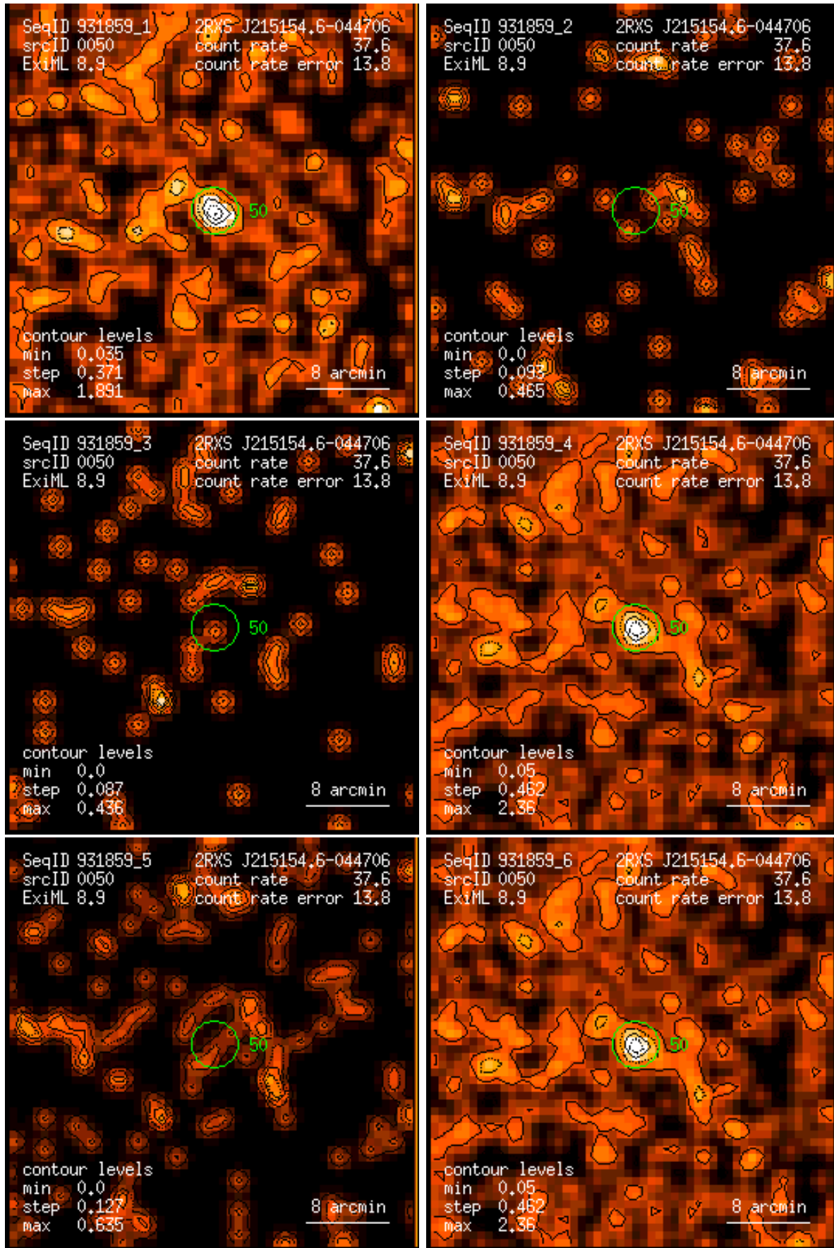
Figure 50: RASS 931859: detection 0050: band rate images, Gaussian filter: (1) PSPC channels 11 – 41, (2) 52 – 90, (3) 91 – 201, (4) 11 – 235, (5) 52 – 201, (6) 11 – 201. Broad band rates in counts/ks. Band rate contour levels in counts/ks/arcmin 2 .
