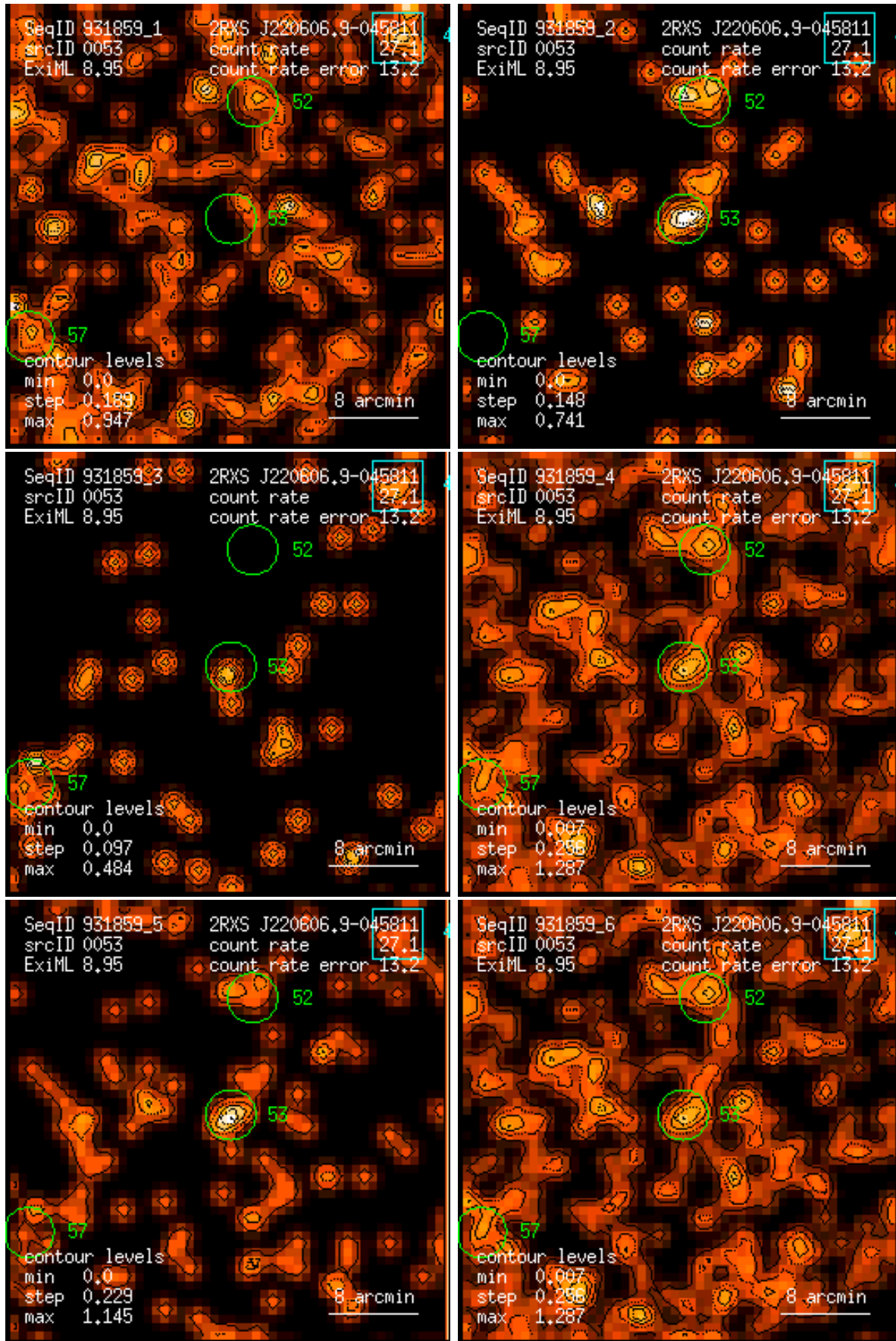
Figure 53: RASS 931859: detection 0053: band rate images, Gaussian filter: (1) PSPC channels 11 – 41, (2) 52 – 90, (3) 91 – 201, (4) 11 – 235, (5) 52 – 201, (6) 11 – 201. Broad band rates in counts/ks. Band rate contour levels in counts/ks/arcmin 2 .
