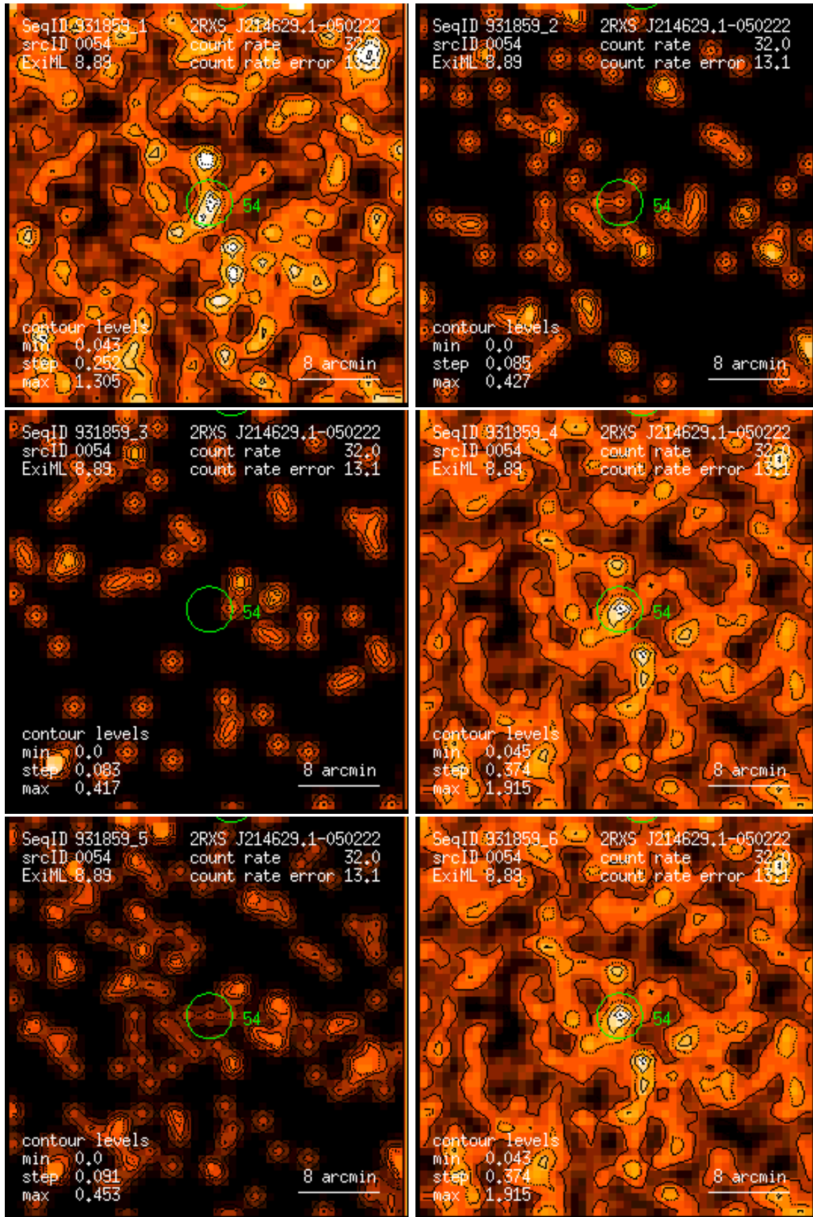
Figure 54: RASS 931859: detection 0054: band rate images, Gaussian filter: (1) PSPC channels 11 – 41, (2) 52 – 90, (3) 91 – 201, (4) 11 – 235, (5) 52 – 201, (6) 11 – 201. Broad band rates in counts/ks. Band rate contour levels in counts/ks/arcmin 2 .
