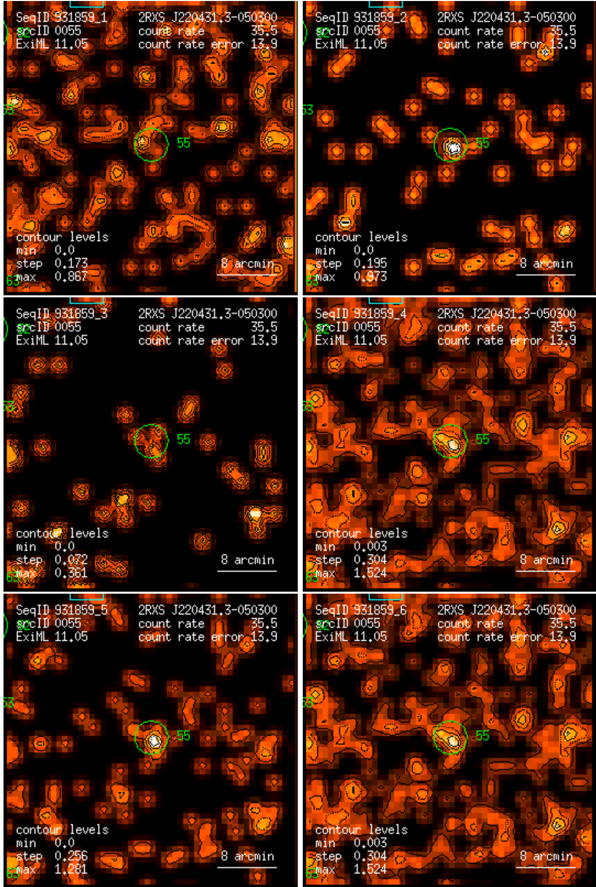
Figure 55: RASS 931859: detection 0055: band rate images, Gaussian filter: (1) PSPC channels 11 – 41, (2) 52 – 90, (3) 91 – 201, (4) 11 – 235, (5) 52 – 201, (6) 11 – 201. Broad band rates in counts/ks. Band rate contour levels in counts/ks/arcmin 2 .
