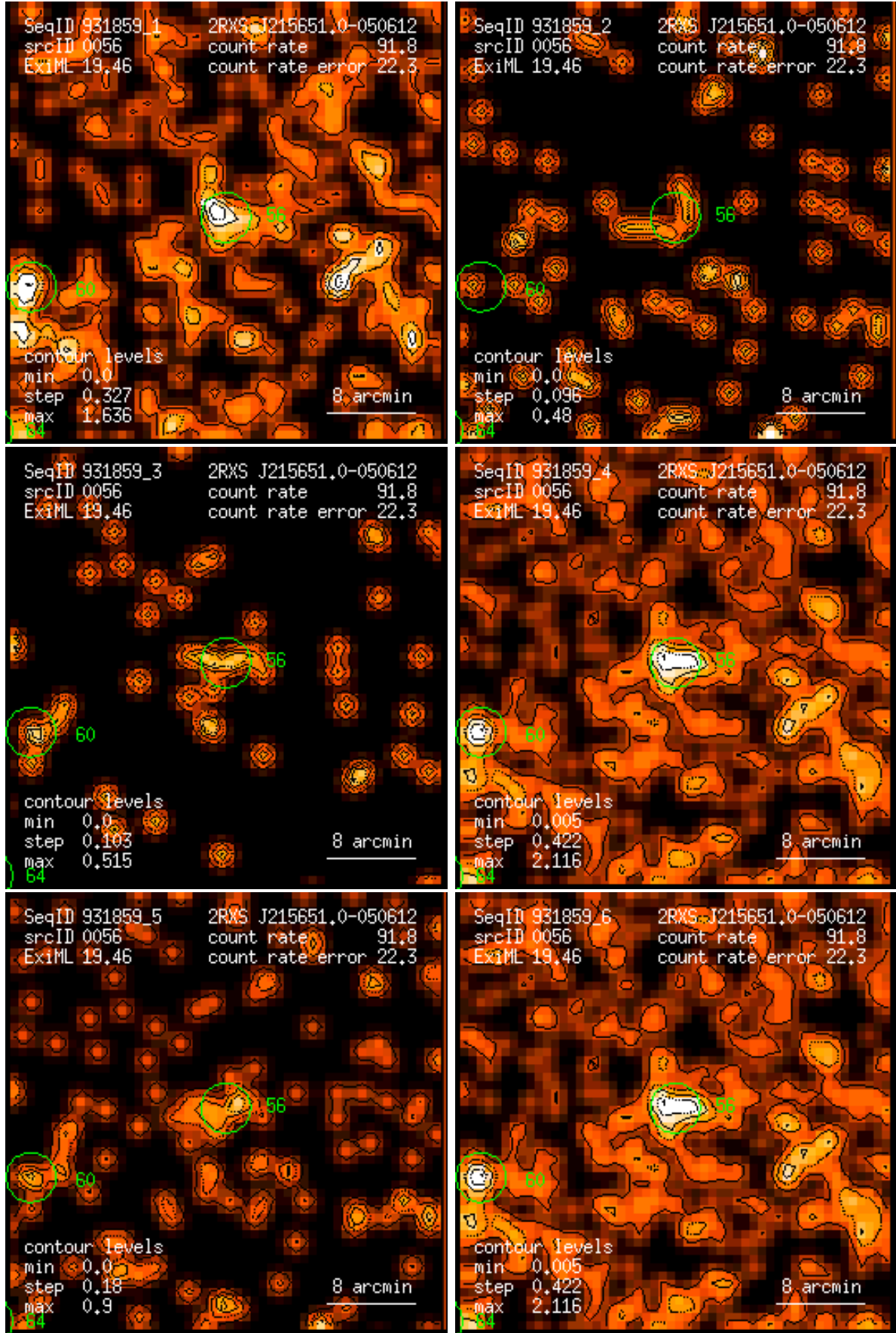
Figure 56: RASS 931859: detection 0056: band rate images, Gaussian filter: (1) PSPC channels 11 – 41, (2) 52 – 90, (3) 91 – 201, (4) 11 – 235, (5) 52 – 201, (6) 11 – 201. Broad band rates in counts/ks. Band rate contour levels in counts/ks/arcmin 2 .
