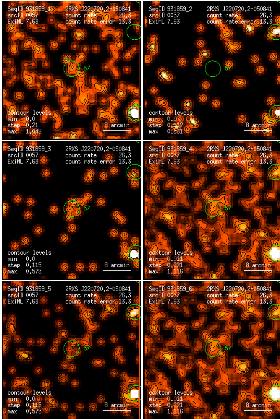
Figure 57: RASS 931859: detection 0057: band rate images, Gaussian filter: (1) PSPC channels 11 – 41, (2) 52 – 90, (3) 91 – 201, (4) 11 – 235, (5) 52 – 201, (6) 11 – 201. Broad band rates in counts/ks. Band rate contour levels in counts/ks/arcmin 2 .
