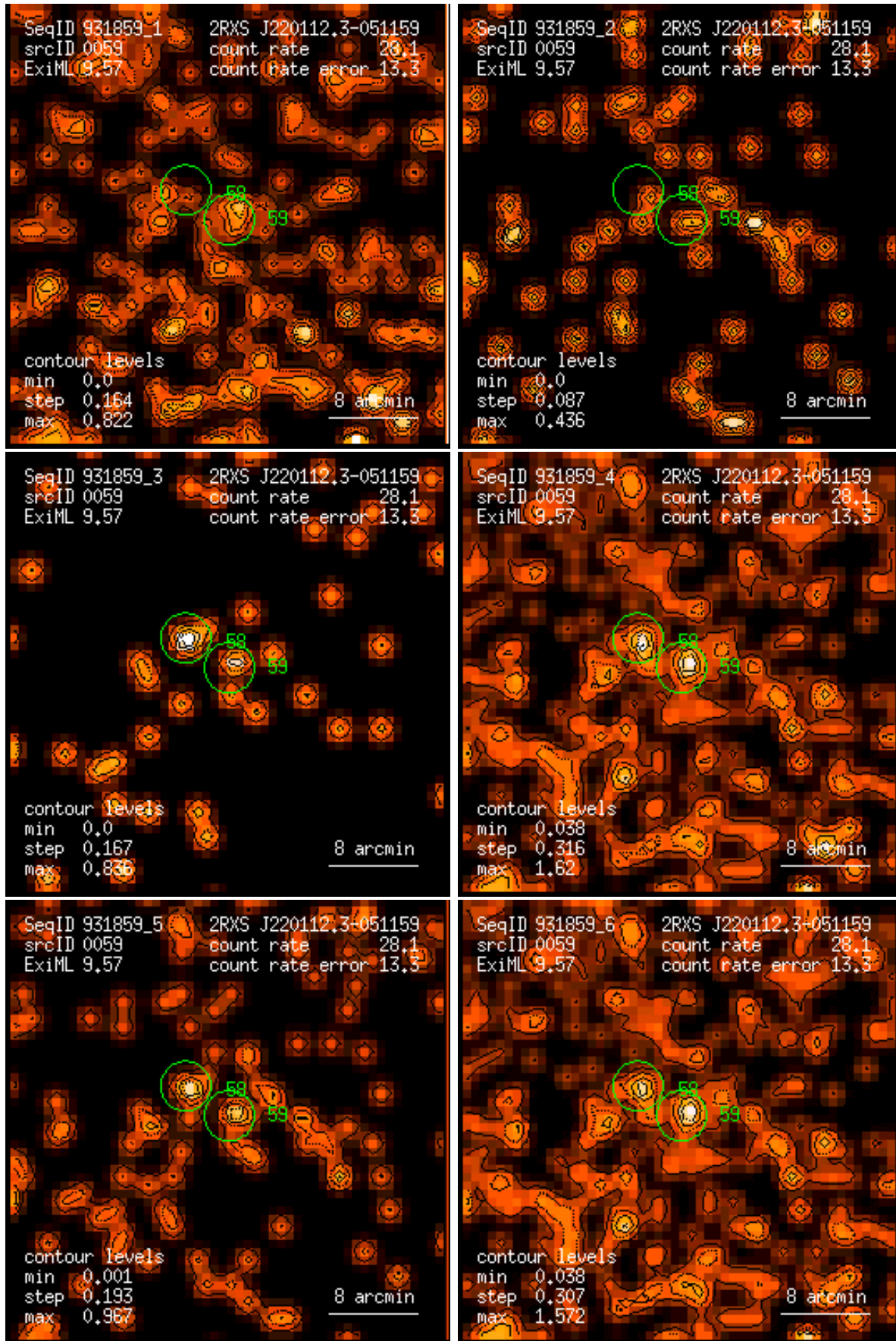
Figure 59: RASS 931859: detection 0059: band rate images, Gaussian filter: (1) PSPC channels 11 – 41, (2) 52 – 90, (3) 91 – 201, (4) 11 – 235, (5) 52 – 201, (6) 11 – 201. Broad band rates in counts/ks. Band rate contour levels in counts/ks/arcmin 2 .
