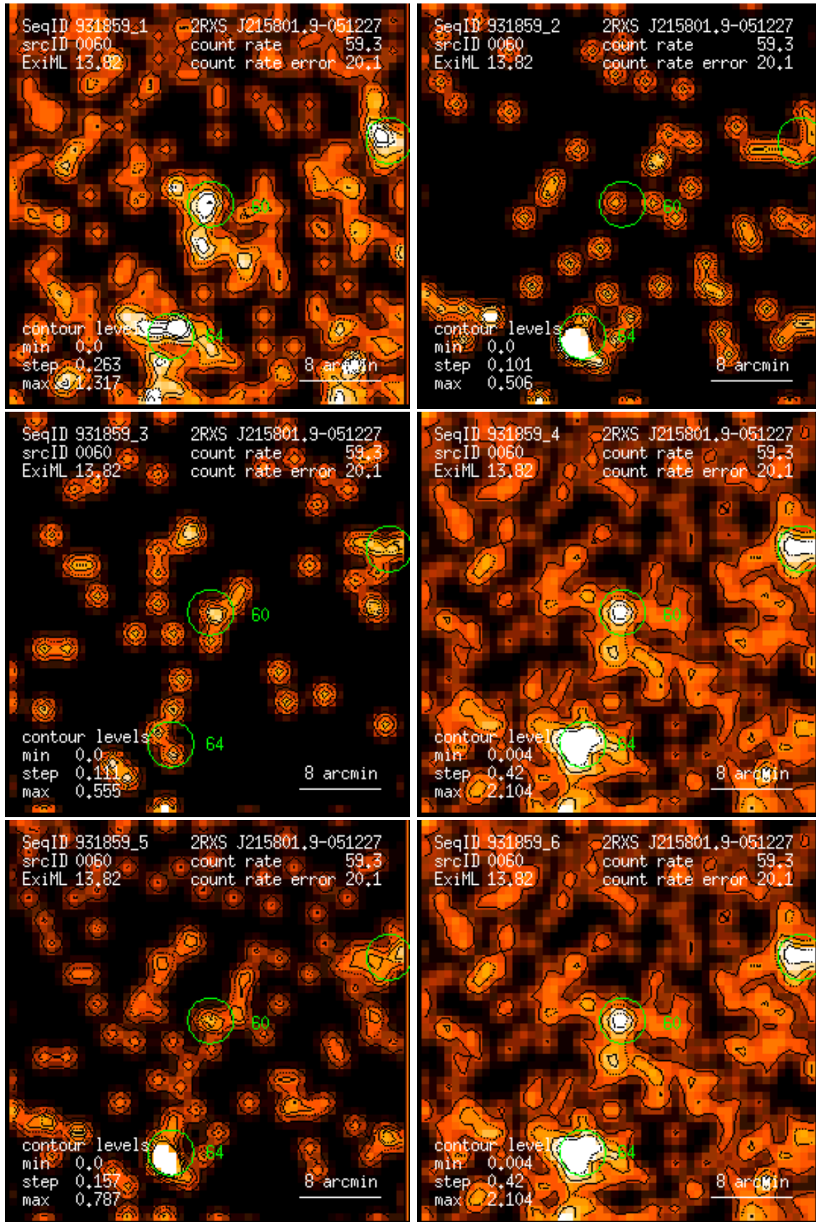
Figure 60: RASS 931859: detection 0060: band rate images, Gaussian filter: (1) PSPC channels 11 – 41, (2) 52 – 90, (3) 91 – 201, (4) 11 – 235, (5) 52 – 201, (6) 11 – 201. Broad band rates in counts/ks. Band rate contour levels in counts/ks/arcmin 2 .
