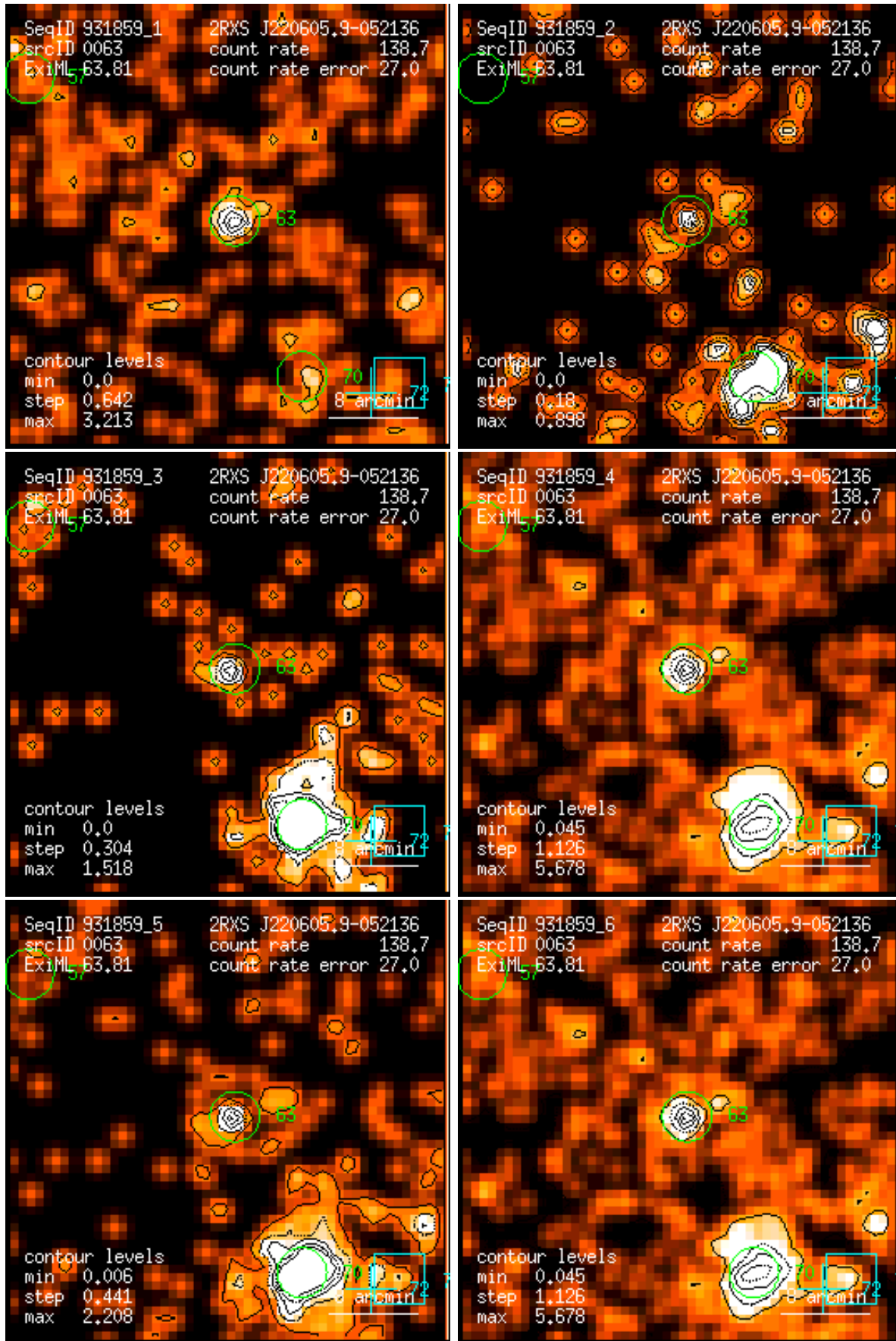
Figure 63: RASS 931859: detection 0063: band rate images, Gaussian filter: (1) PSPC channels 11 – 41, (2) 52 – 90, (3) 91 – 201, (4) 11 – 235, (5) 52 – 201, (6) 11 – 201. Broad band rates in counts/ks. Band rate contour levels in counts/ks/arcmin 2 .
