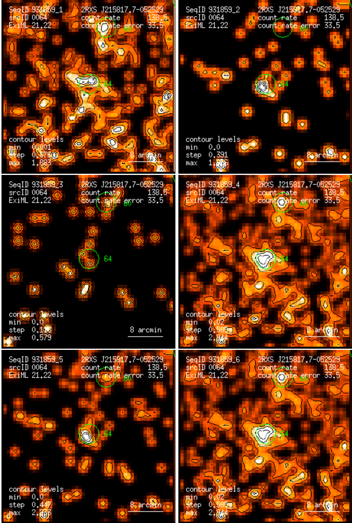
Figure 64: RASS 931859: detection 0064: band rate images, Gaussian filter: (1) PSPC channels 11 – 41, (2) 52 – 90, (3) 91 – 201, (4) 11 – 235, (5) 52 – 201, (6) 11 – 201. Broad band rates in counts/ks. Band rate contour levels in counts/ks/arcmin 2 .
