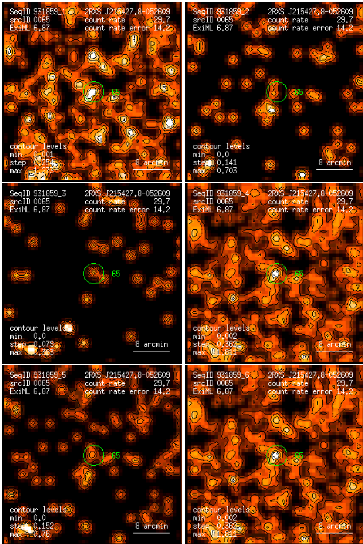
Figure 65: RASS 931859: detection 0065: band rate images, Gaussian filter: (1) PSPC channels 11 – 41, (2) 52 – 90, (3) 91 – 201, (4) 11 – 235, (5) 52 – 201, (6) 11 – 201. Broad band rates in counts/ks. Band rate contour levels in counts/ks/arcmin 2 .
