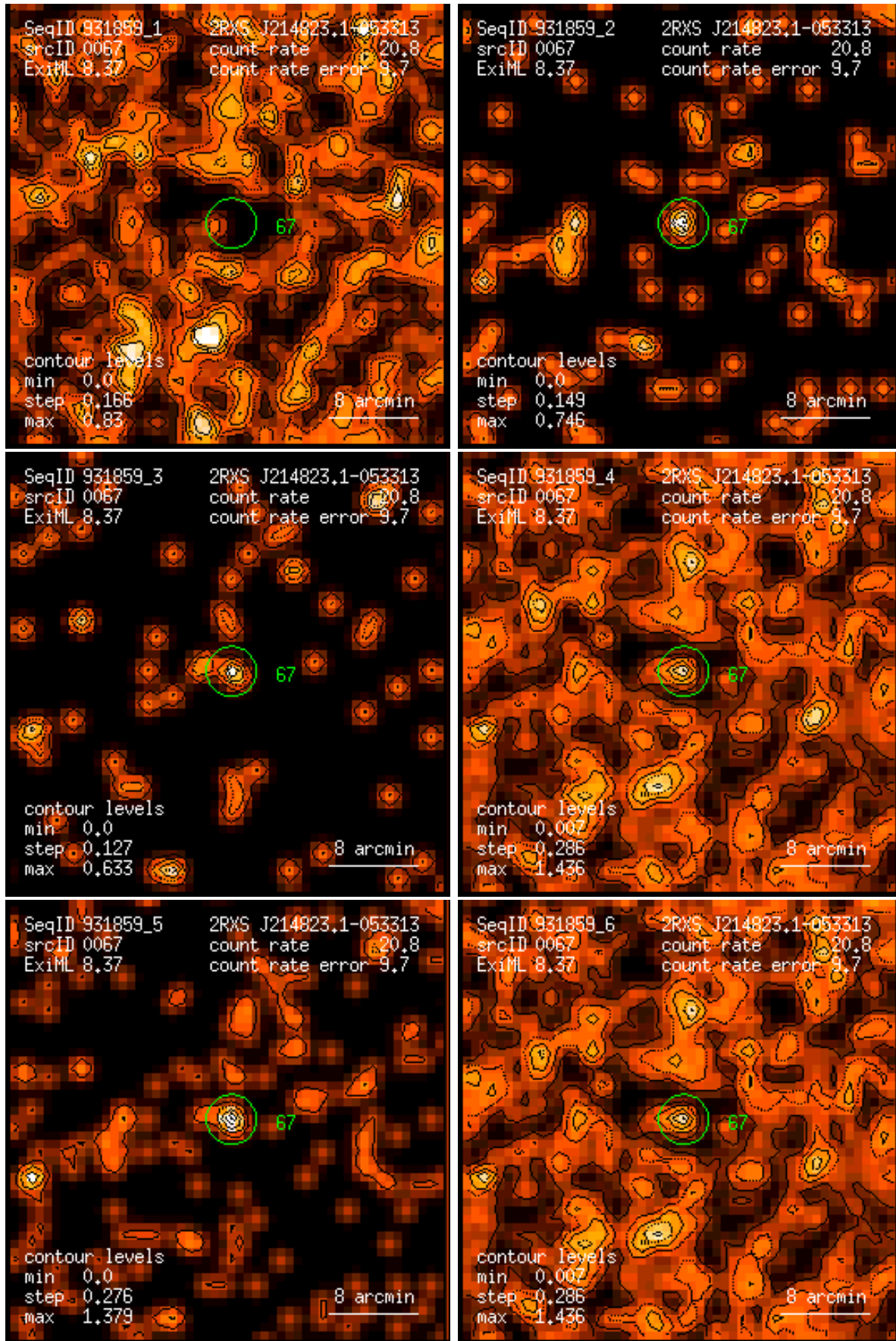
Figure 67: RASS 931859: detection 0067: band rate images, Gaussian filter: (1) PSPC channels 11 – 41, (2) 52 – 90, (3) 91 – 201, (4) 11 – 235, (5) 52 – 201, (6) 11 – 201. Broad band rates in counts/ks. Band rate contour levels in counts/ks/arcmin 2 .
