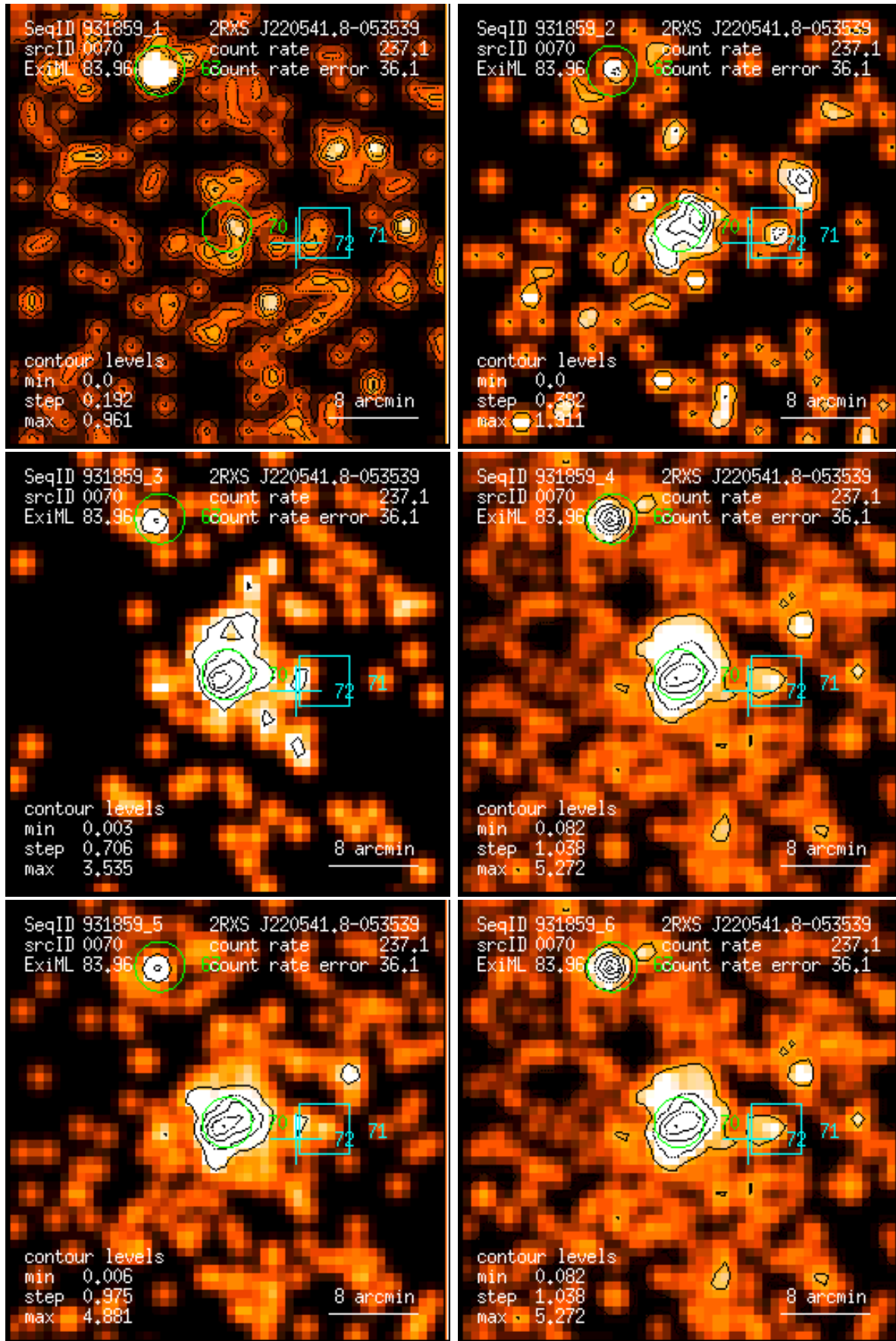
Figure 70: RASS 931859: detection 0070: band rate images, Gaussian filter: (1) PSPC channels 11 – 41, (2) 52 – 90, (3) 91 – 201, (4) 11 – 235, (5) 52 – 201, (6) 11 – 201. Broad band rates in counts/ks. Band rate contour levels in counts/ks/arcmin 2 .
