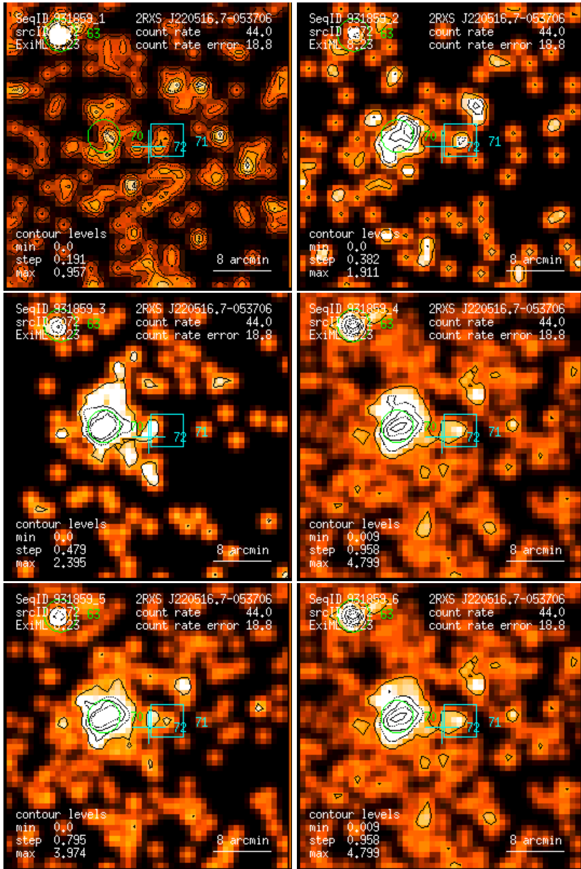
Figure 72: RASS 931859: detection 0072: band rate images, Gaussian filter: (1) PSPC channels 11 – 41, (2) 52 – 90, (3) 91 – 201, (4) 11 – 235, (5) 52 – 201, (6) 11 – 201. Broad band rates in counts/ks. Band rate contour levels in counts/ks/arcmin 2 .
