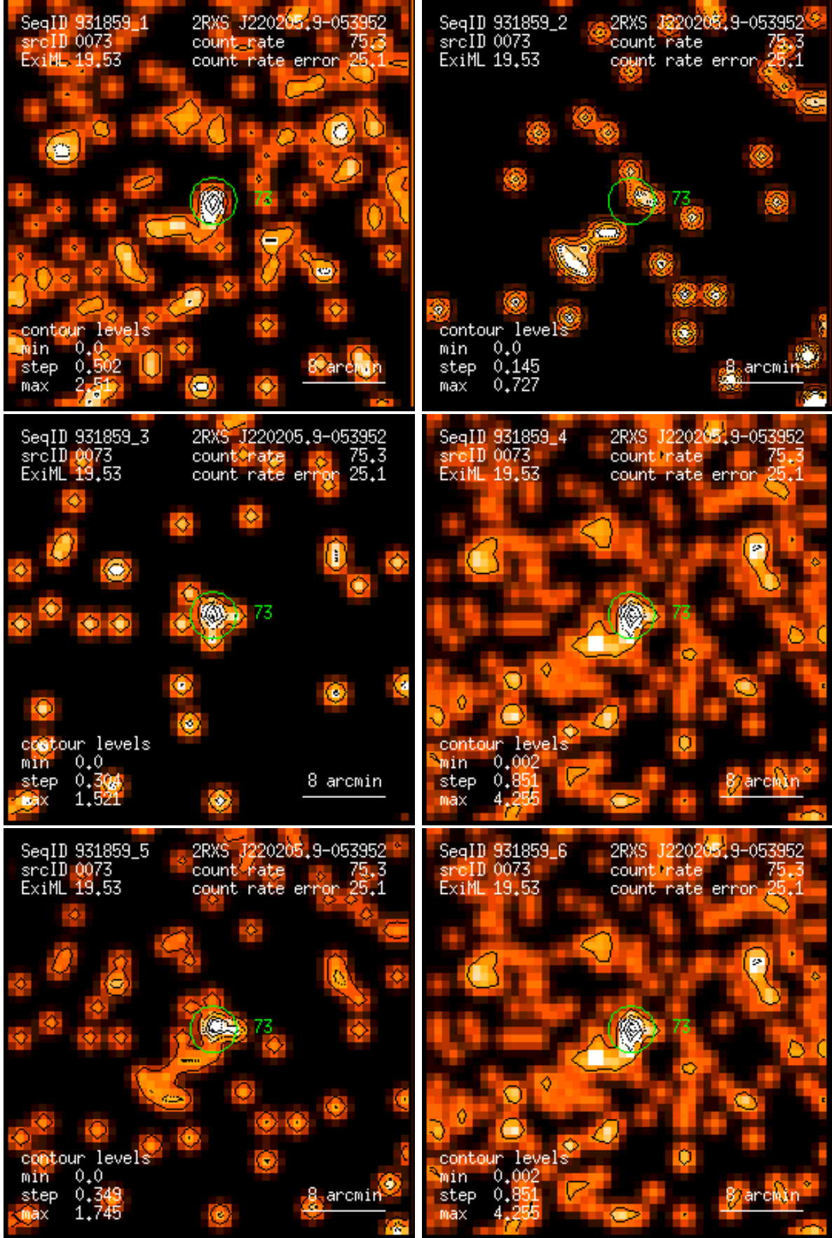
Figure 73: RASS 931859: detection 0073: band rate images, Gaussian filter: (1) PSPC channels 11 – 41, (2) 52 – 90, (3) 91 – 201, (4) 11 – 235, (5) 52 – 201, (6) 11 – 201. Broad band rates in counts/ks. Band rate contour levels in counts/ks/arcmin 2 .
