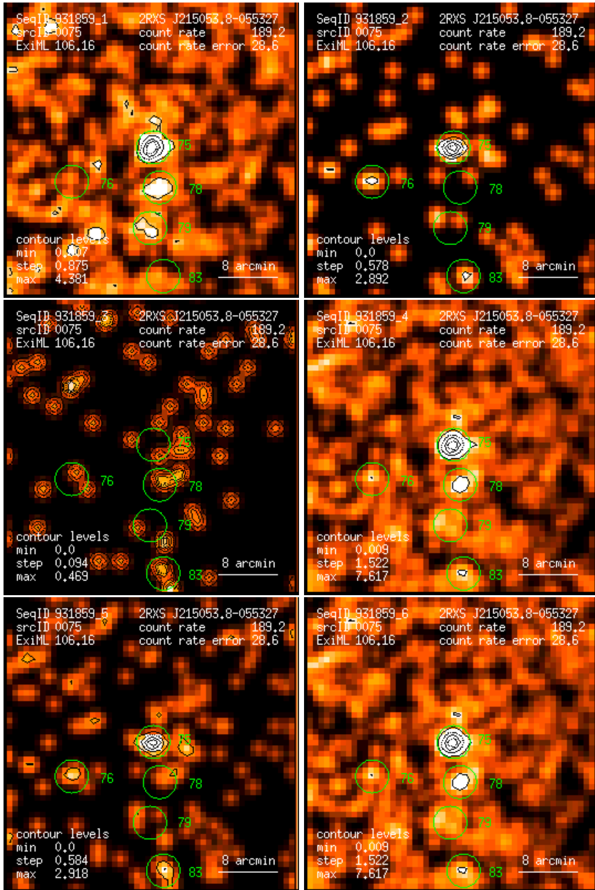
Figure 75: RASS 931859: detection 0075: band rate images, Gaussian filter: (1) PSPC channels 11 – 41, (2) 52 – 90, (3) 91 – 201, (4) 11 – 235, (5) 52 – 201, (6) 11 – 201. Broad band rates in counts/ks. Band rate contour levels in counts/ks/arcmin 2 .
