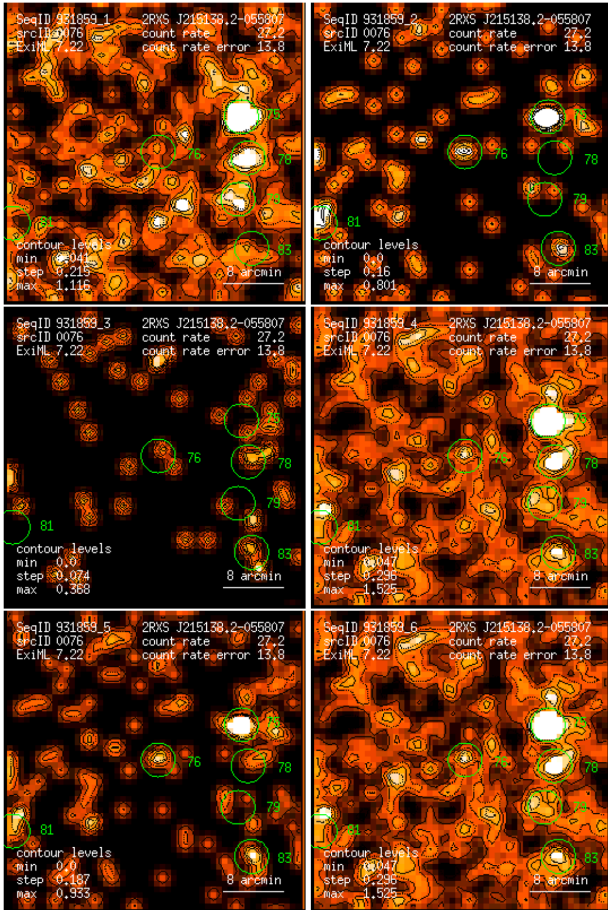
Figure 76: RASS 931859: detection 0076: band rate images, Gaussian filter: (1) PSPC channels 11 – 41, (2) 52 – 90, (3) 91 – 201, (4) 11 – 235, (5) 52 – 201, (6) 11 – 201. Broad band rates in counts/ks. Band rate contour levels in counts/ks/arcmin 2 .
