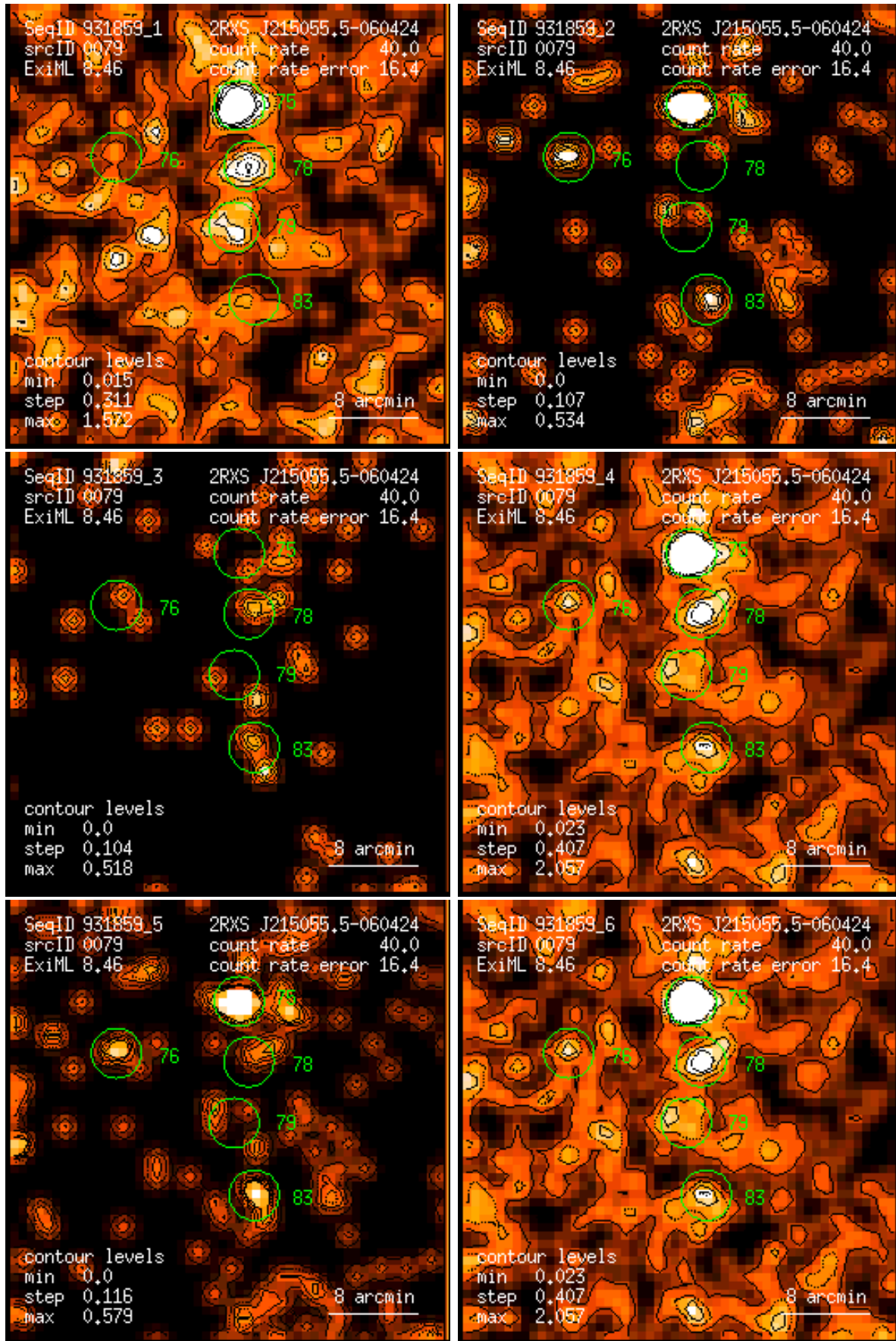
Figure 79: RASS 931859: detection 0079: band rate images, Gaussian filter: (1) PSPC channels 11 – 41, (2) 52 – 90, (3) 91 – 201, (4) 11 – 235, (5) 52 – 201, (6) 11 – 201. Broad band rates in counts/ks. Band rate contour levels in counts/ks/arcmin 2 .
