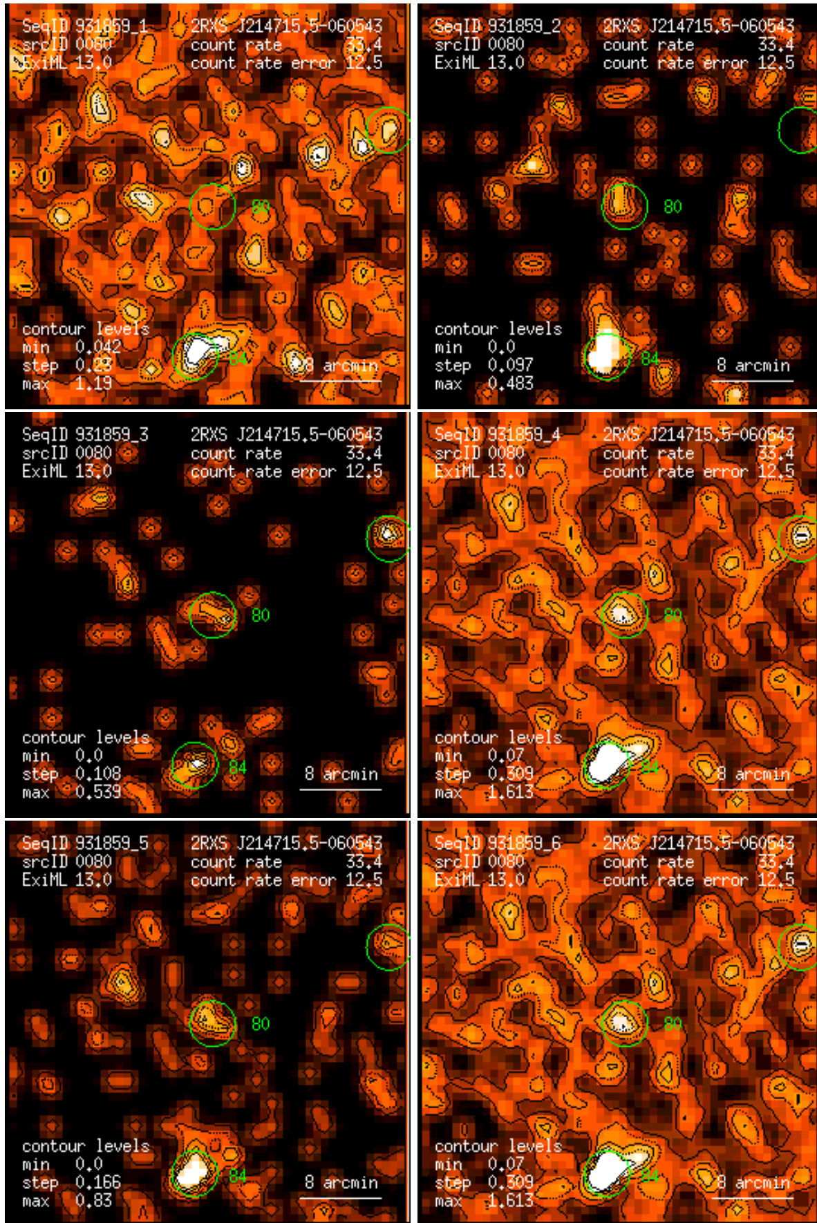
Figure 80: RASS 931859: detection 0080: band rate images, Gaussian filter: (1) PSPC channels 11 – 41, (2) 52 – 90, (3) 91 – 201, (4) 11 – 235, (5) 52 – 201, (6) 11 – 201. Broad band rates in counts/ks. Band rate contour levels in counts/ks/arcmin 2 .
