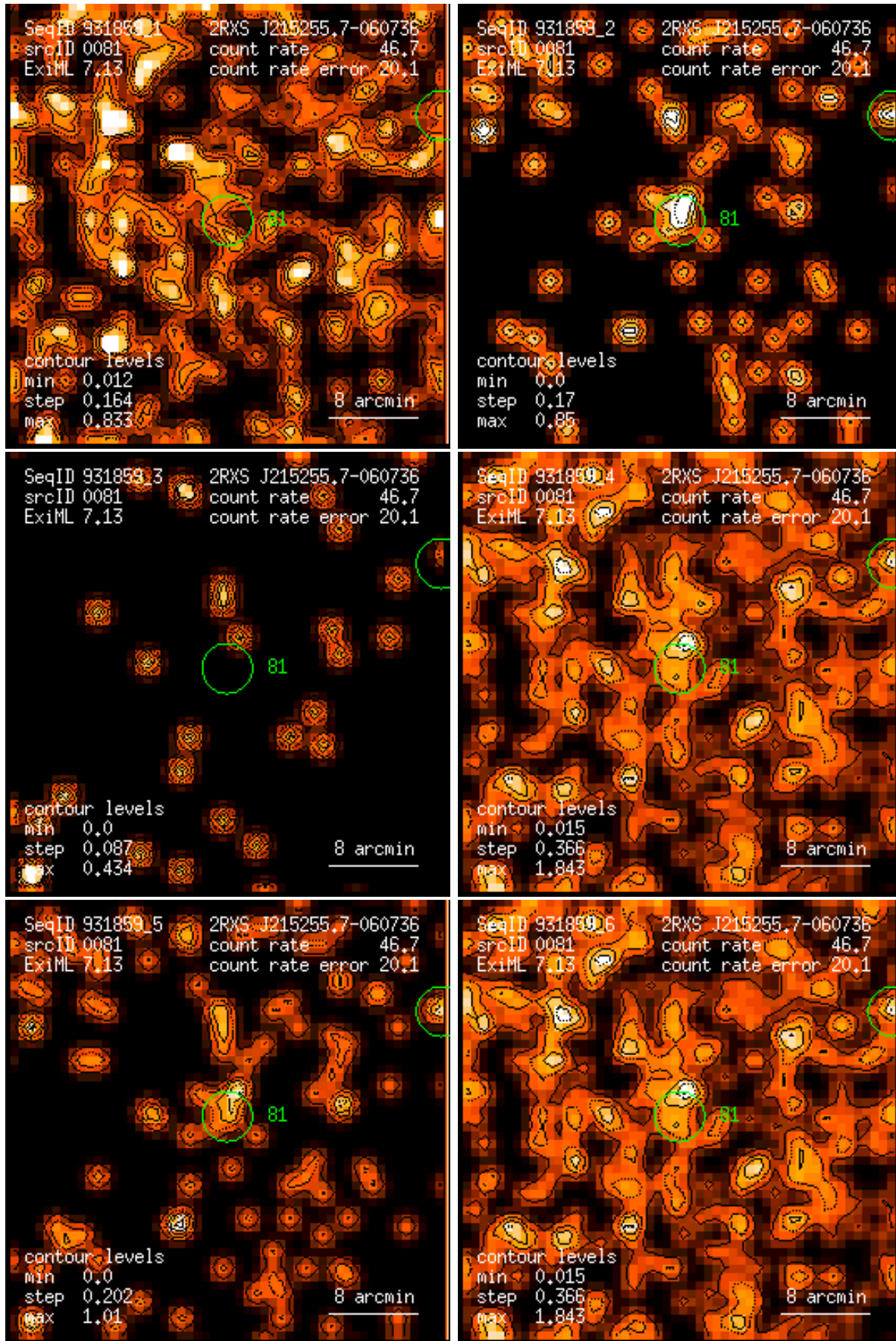
Figure 81: RASS 931859: detection 0081: band rate images, Gaussian filter: (1) PSPC channels 11 – 41, (2) 52 – 90, (3) 91 – 201, (4) 11 – 235, (5) 52 – 201, (6) 11 – 201. Broad band rates in counts/ks. Band rate contour levels in counts/ks/arcmin 2 .
