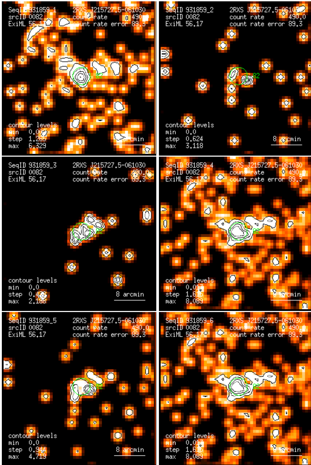
Figure 82: RASS 931859: detection 0082: band rate images, Gaussian filter: (1) PSPC channels 11 – 41, (2) 52 – 90, (3) 91 – 201, (4) 11 – 235, (5) 52 – 201, (6) 11 – 201. Broad band rates in counts/ks. Band rate contour levels in counts/ks/arcmin 2 .
