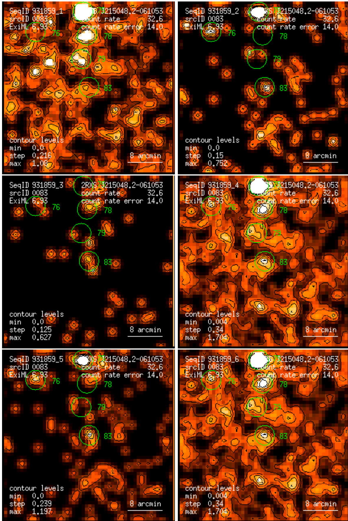
Figure 83: RASS 931859: detection 0083: band rate images, Gaussian filter: (1) PSPC channels 11 – 41, (2) 52 – 90, (3) 91 – 201, (4) 11 – 235, (5) 52 – 201, (6) 11 – 201. Broad band rates in counts/ks. Band rate contour levels in counts/ks/arcmin 2 .
