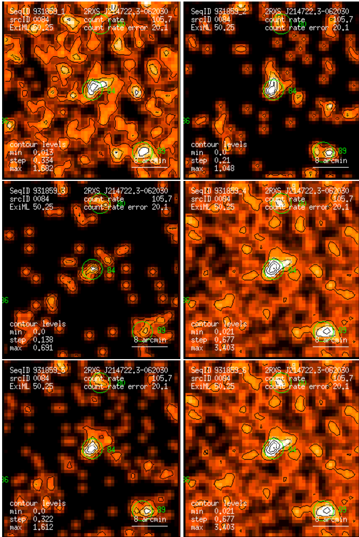
Figure 84: RASS 931859: detection 0084: band rate images, Gaussian filter: (1) PSPC channels 11 – 41, (2) 52 – 90, (3) 91 – 201, (4) 11 – 235, (5) 52 – 201, (6) 11 – 201. Broad band rates in counts/ks. Band rate contour levels in counts/ks/arcmin 2 .
