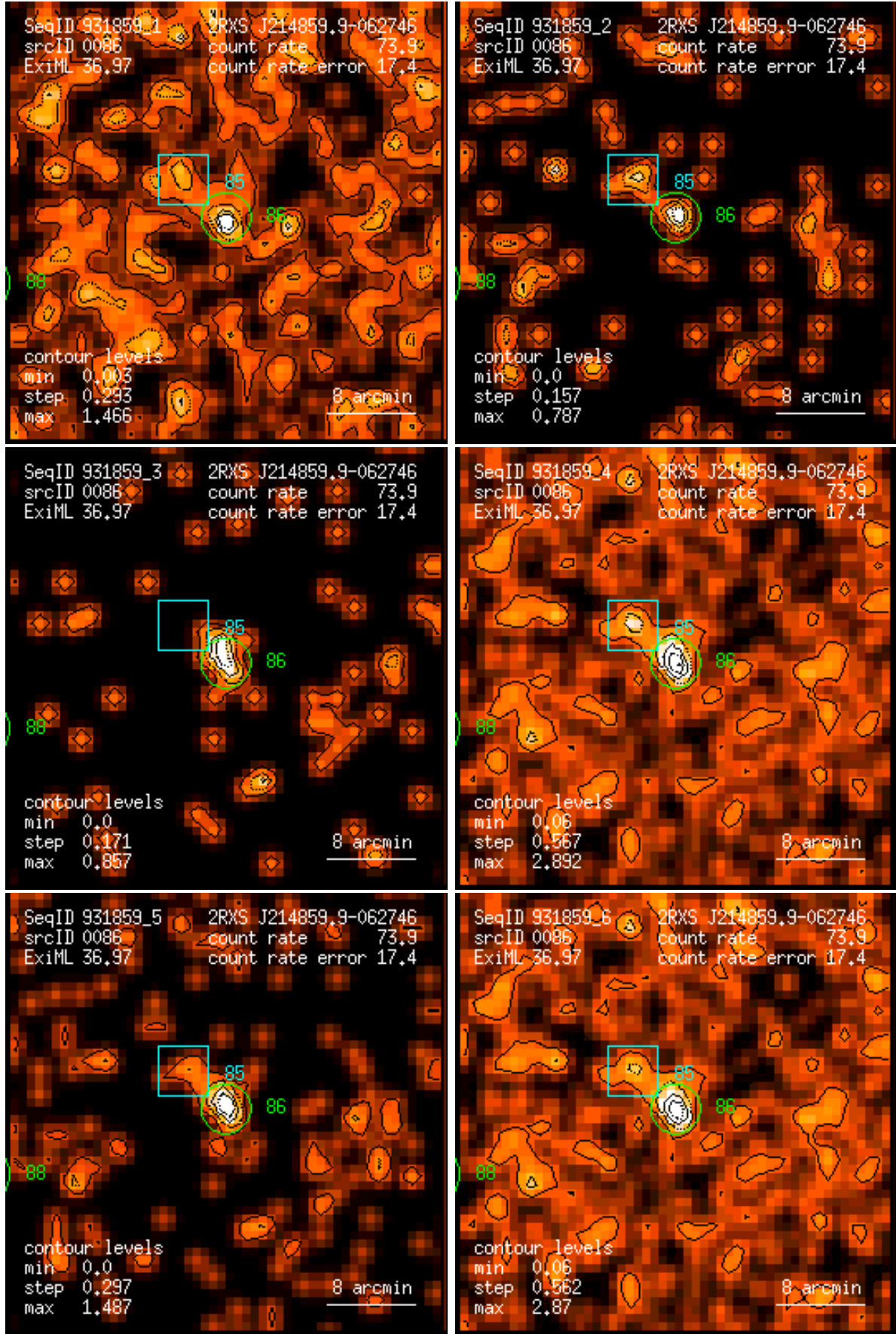
Figure 86: RASS 931859: detection 0086: band rate images, Gaussian filter: (1) PSPC channels 11 – 41, (2) 52 – 90, (3) 91 – 201, (4) 11 – 235, (5) 52 – 201, (6) 11 – 201. Broad band rates in counts/ks. Band rate contour levels in counts/ks/arcmin 2 .
