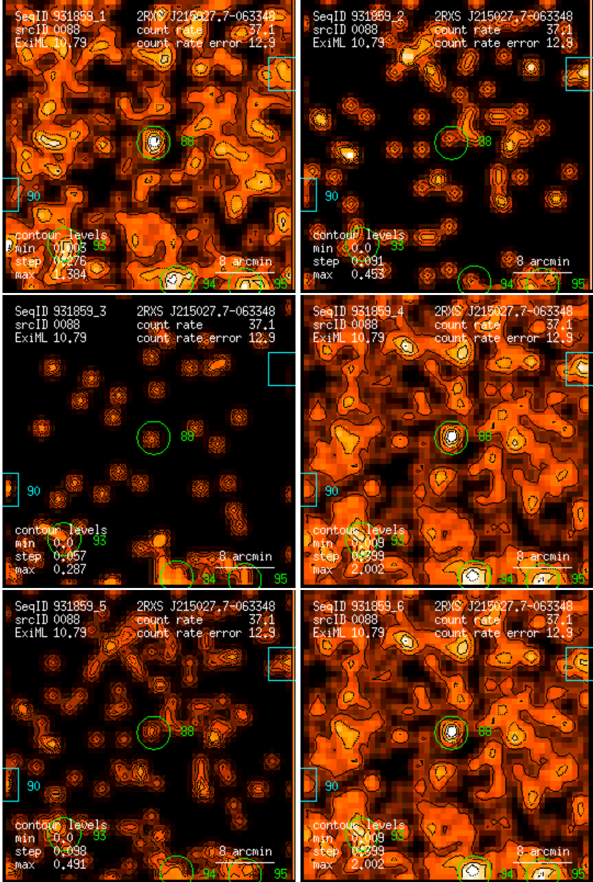
Figure 88: RASS 931859: detection 0088: band rate images, Gaussian filter: (1) PSPC channels 11 – 41, (2) 52 – 90, (3) 91 – 201, (4) 11 – 235, (5) 52 – 201, (6) 11 – 201. Broad band rates in counts/ks. Band rate contour levels in counts/ks/arcmin 2 .
