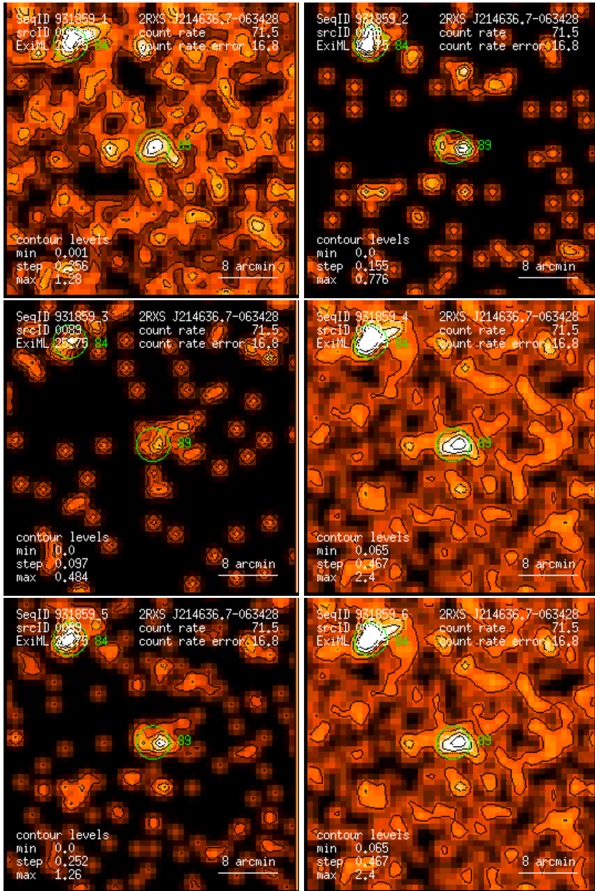
Figure 89: RASS 931859: detection 0089: band rate images, Gaussian filter: (1) PSPC channels 11 – 41, (2) 52 – 90, (3) 91 – 201, (4) 11 – 235, (5) 52 – 201, (6) 11 – 201. Broad band rates in counts/ks. Band rate contour levels in counts/ks/arcmin 2 .
