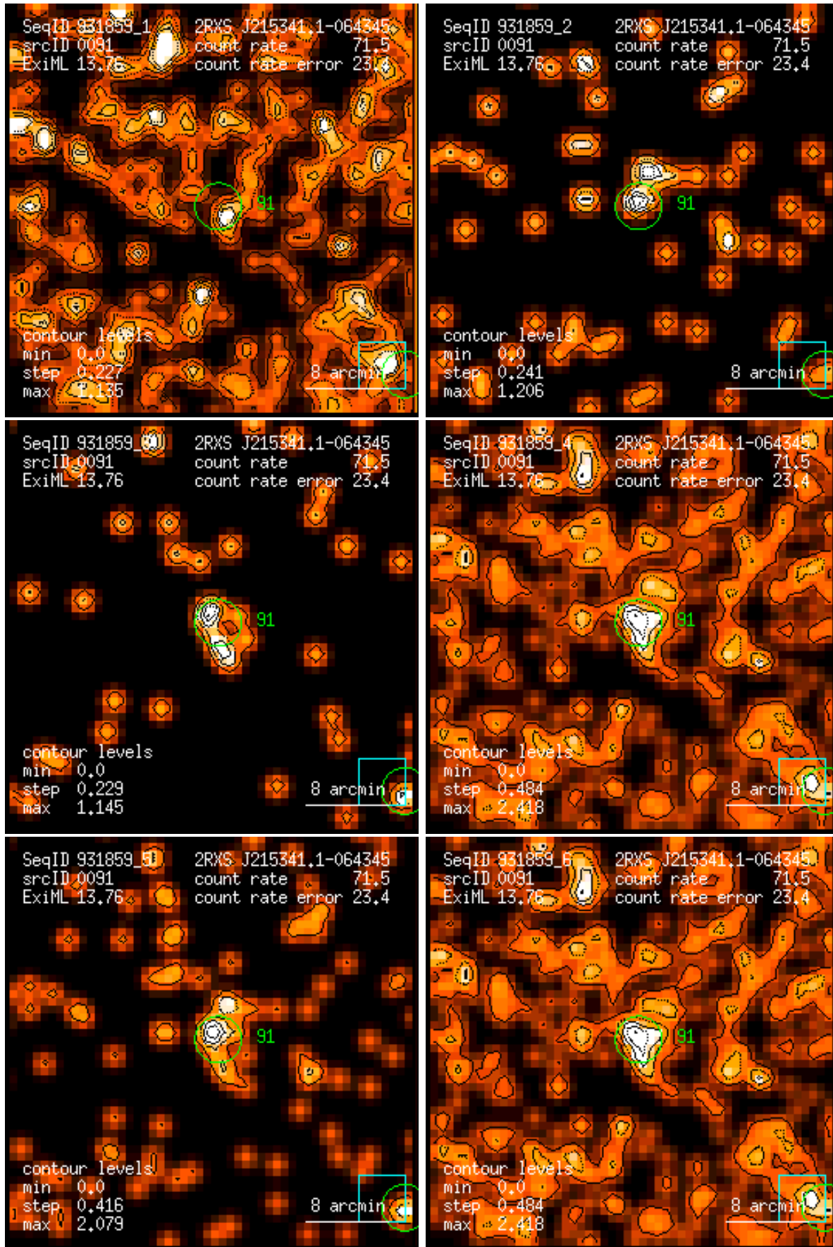
Figure 91: RASS 931859: detection 0091: band rate images, Gaussian filter: (1) PSPC channels 11 – 41, (2) 52 – 90, (3) 91 – 201, (4) 11 – 235, (5) 52 – 201, (6) 11 – 201. Broad band rates in counts/ks. Band rate contour levels in counts/ks/arcmin 2 .
