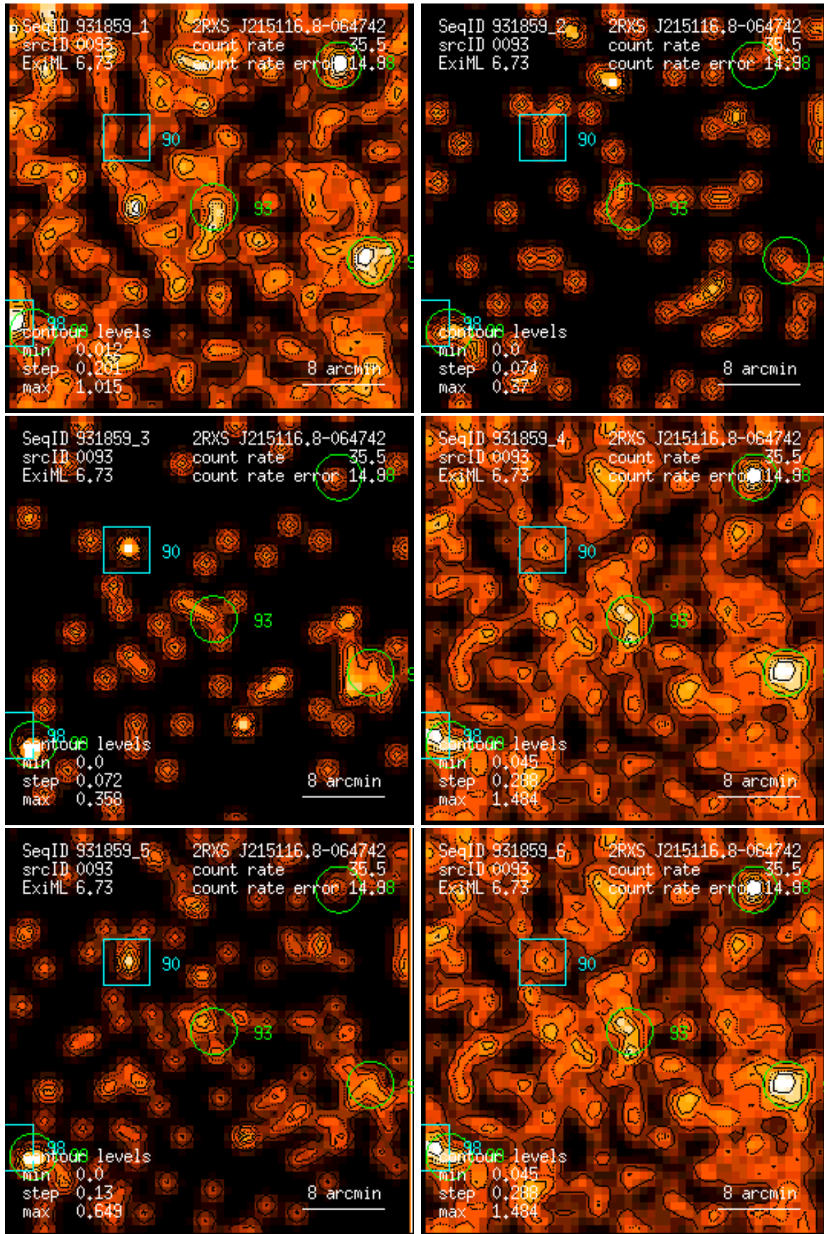
Figure 93: RASS 931859: detection 0093: band rate images, Gaussian filter: (1) PSPC channels 11 – 41, (2) 52 – 90, (3) 91 – 201, (4) 11 – 235, (5) 52 – 201, (6) 11 – 201. Broad band rates in counts/ks. Band rate contour levels in counts/ks/arcmin 2 .
