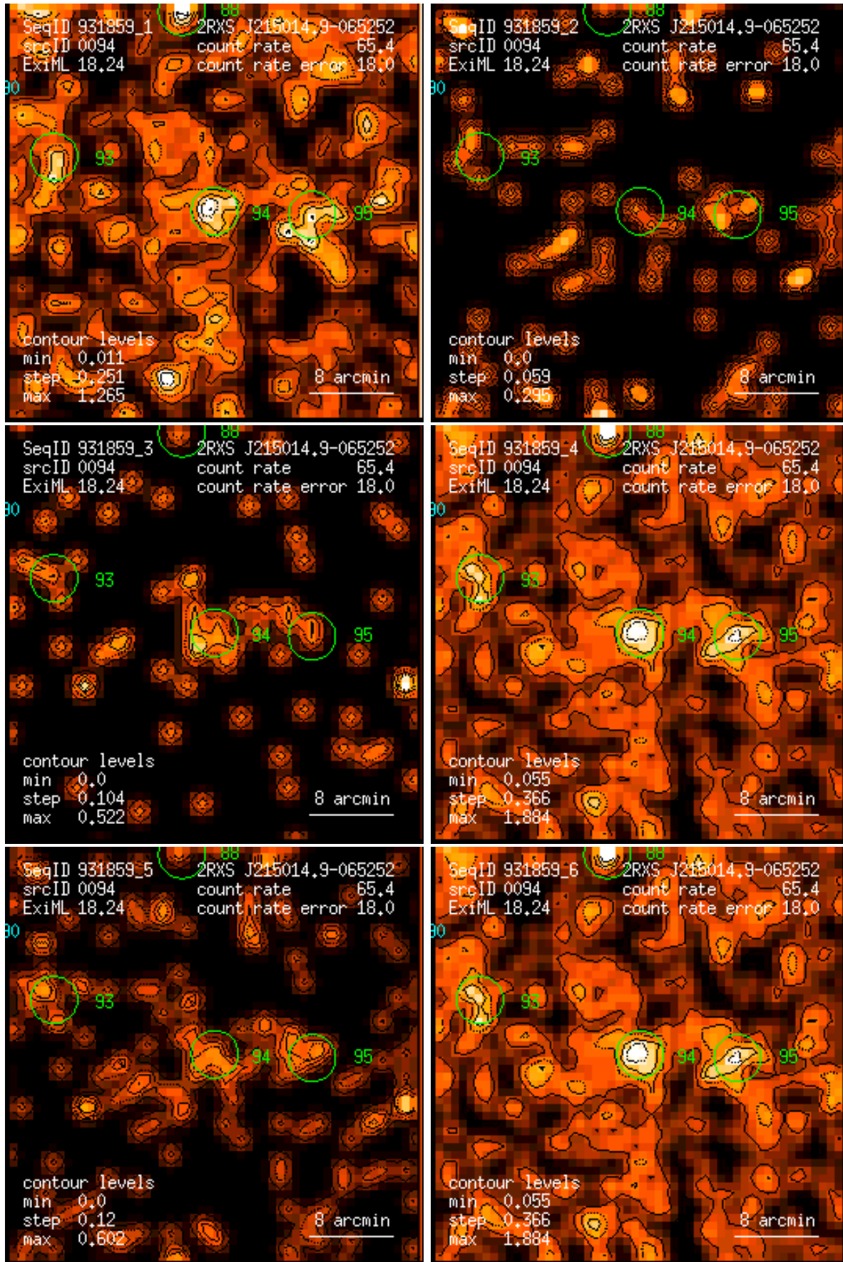
Figure 94: RASS 931859: detection 0094: band rate images, Gaussian filter: (1) PSPC channels 11 – 41, (2) 52 – 90, (3) 91 – 201, (4) 11 – 235, (5) 52 – 201, (6) 11 – 201. Broad band rates in counts/ks. Band rate contour levels in counts/ks/arcmin 2 .
