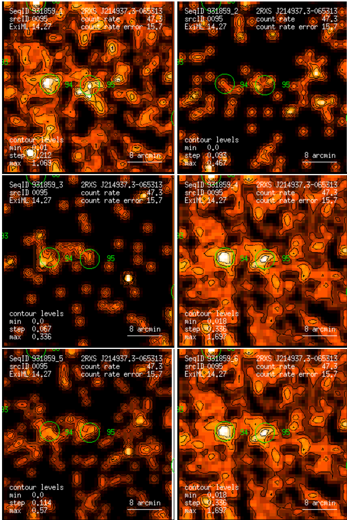
Figure 95: RASS 931859: detection 0095: band rate images, Gaussian filter: (1) PSPC channels 11 – 41, (2) 52 – 90, (3) 91 – 201, (4) 11 – 235, (5) 52 – 201, (6) 11 – 201. Broad band rates in counts/ks. Band rate contour levels in counts/ks/arcmin 2 .
