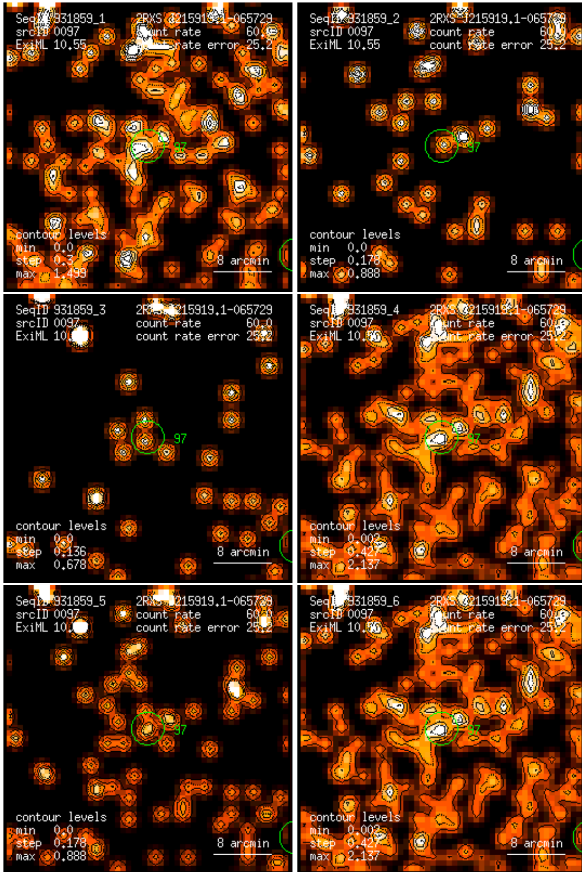
Figure 97: RASS 931859: detection 0097: band rate images, Gaussian filter: (1) PSPC channels 11 – 41, (2) 52 – 90, (3) 91 – 201, (4) 11 – 235, (5) 52 – 201, (6) 11 – 201. Broad band rates in counts/ks. Band rate contour levels in counts/ks/arcmin 2 .
