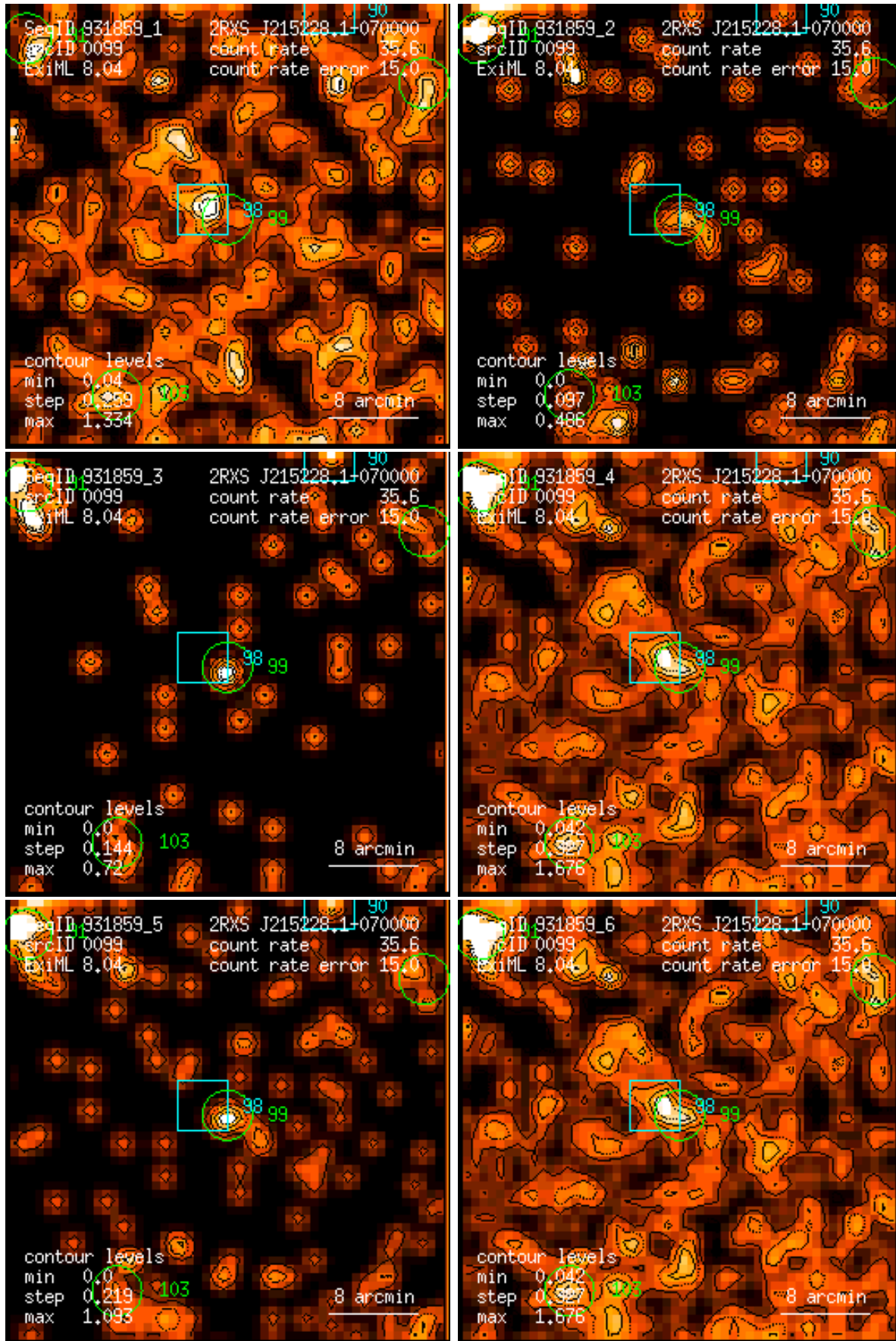
Figure 99: RASS 931859: detection 0099: band rate images, Gaussian filter: (1) PSPC channels 11 – 41, (2) 52 – 90, (3) 91 – 201, (4) 11 – 235, (5) 52 – 201, (6) 11 – 201. Broad band rates in counts/ks. Band rate contour levels in counts/ks/arcmin 2 .
